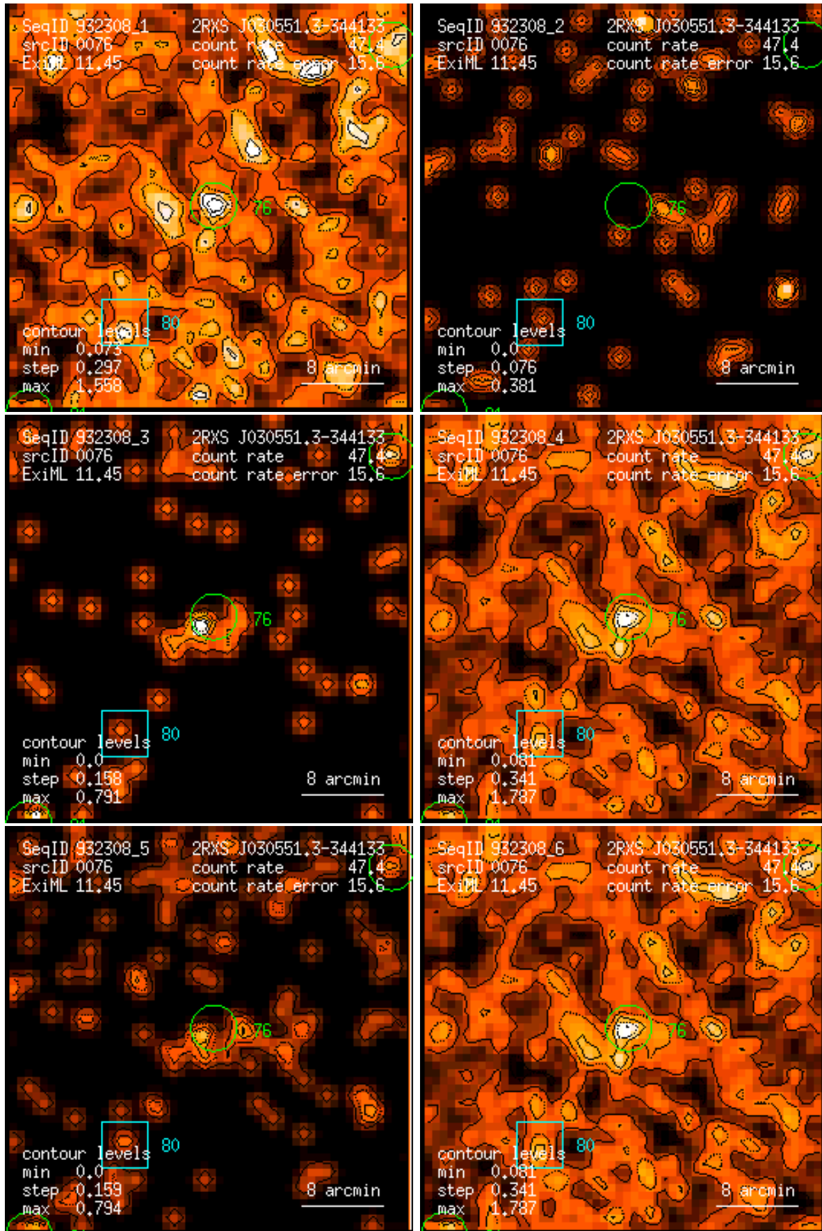
Figure 76: RASS 932308: detection 0076: band rate images, Gaussian filter: (1) PSPC channels 11 – 41, (2) 52 – 90, (3) 91 – 201, (4) 11 – 235, (5) 52 – 201, (6) 11 – 201. Broad band rates in counts/ks. Band rate contour levels in counts/ks/arcmin 2 .
