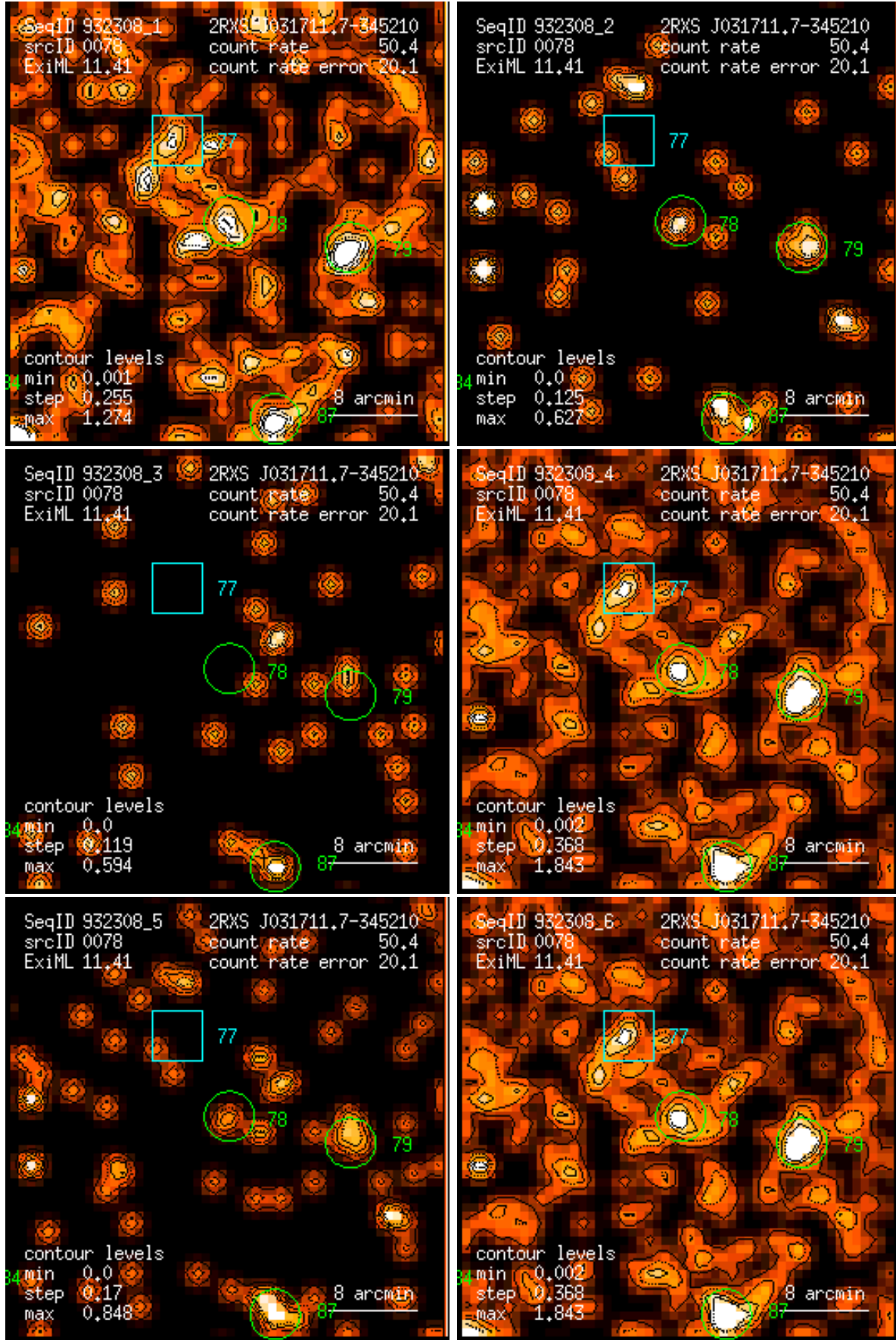
Figure 78: RASS 932308: detection 0078: band rate images, Gaussian filter: (1) PSPC channels 11 – 41, (2) 52 – 90, (3) 91 – 201, (4) 11 – 235, (5) 52 – 201, (6) 11 – 201. Broad band rates in counts/ks. Band rate contour levels in counts/ks/arcmin 2 .
