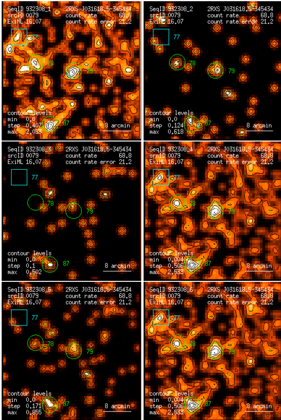
Figure 79: RASS 932308: detection 0079: band rate images, Gaussian filter: (1) PSPC channels 11 – 41, (2) 52 – 90, (3) 91 – 201, (4) 11 – 235, (5) 52 – 201, (6) 11 – 201. Broad band rates in counts/ks. Band rate contour levels in counts/ks/arcmin 2 .
