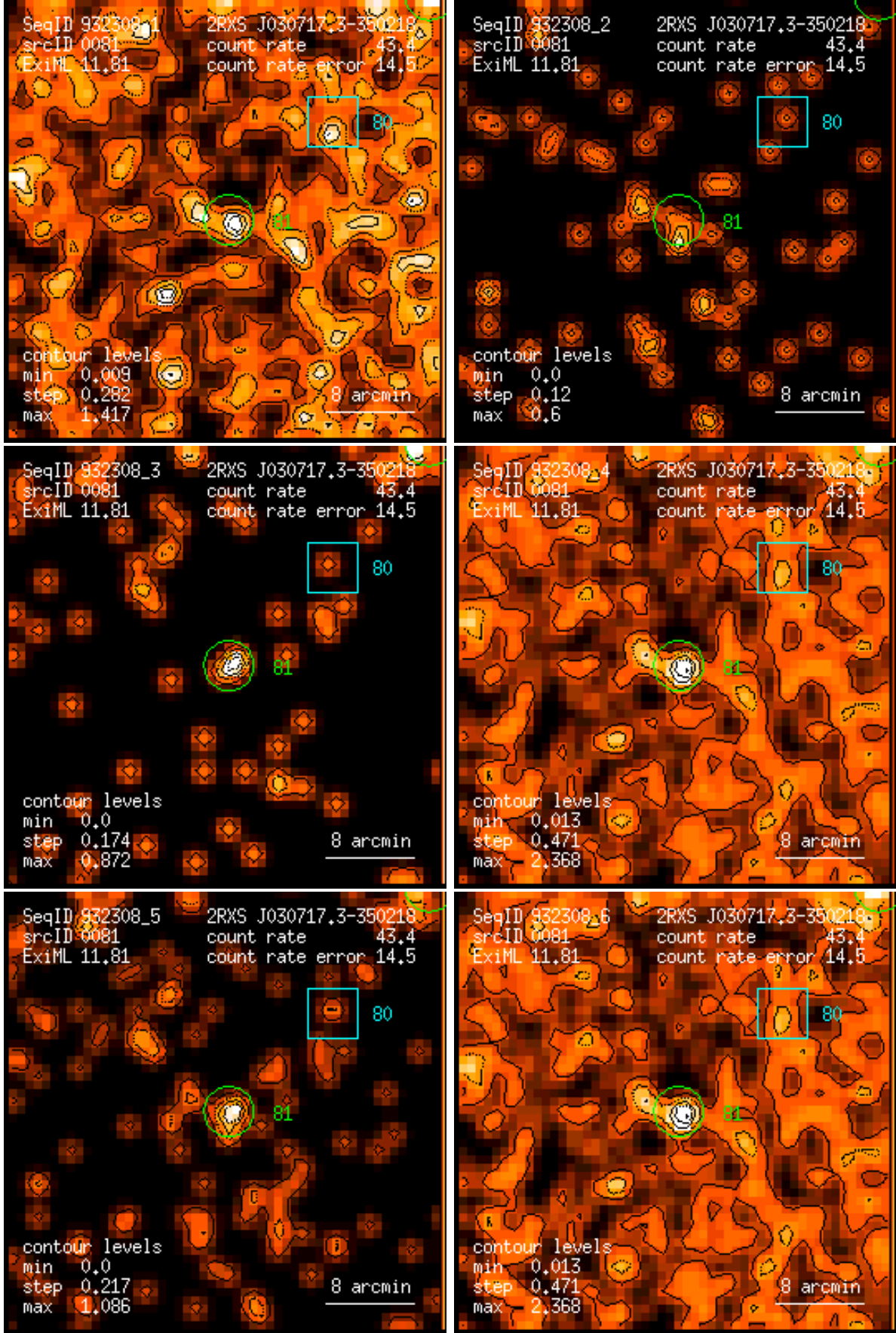
Figure 81: RASS 932308: detection 0081: band rate images, Gaussian filter: (1) PSPC channels 11 – 41, (2) 52 – 90, (3) 91 – 201, (4) 11 – 235, (5) 52 – 201, (6) 11 – 201. Broad band rates in counts/ks. Band rate contour levels in counts/ks/arcmin 2 .
