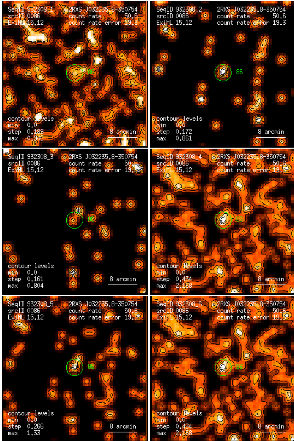
Figure 86: RASS 932308: detection 0086: band rate images, Gaussian filter: (1) PSPC channels 11 – 41, (2) 52 – 90, (3) 91 – 201, (4) 11 – 235, (5) 52 – 201, (6) 11 – 201. Broad band rates in counts/ks. Band rate contour levels in counts/ks/arcmin 2 .
