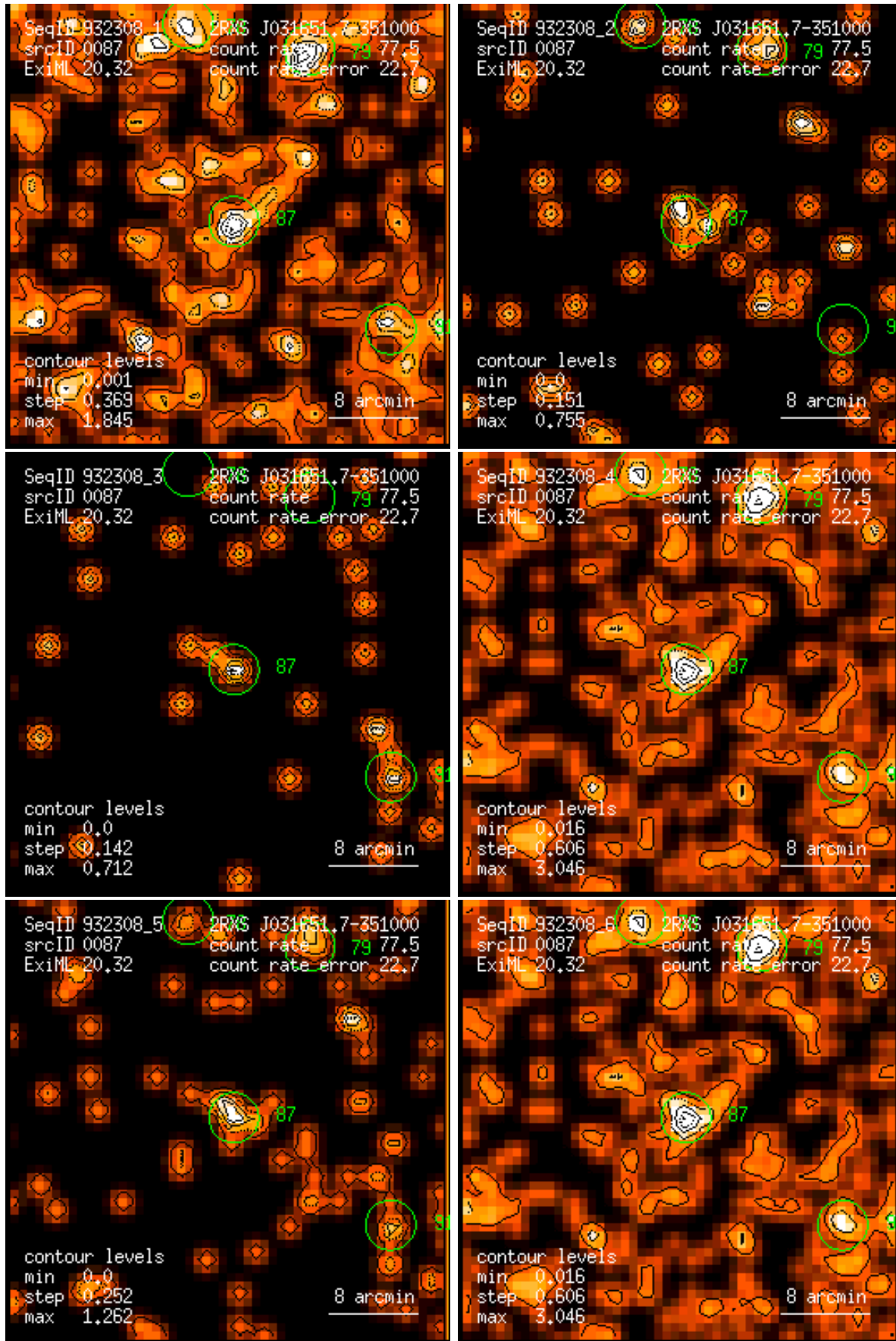
Figure 87: RASS 932308: detection 0087: band rate images, Gaussian filter: (1) PSPC channels 11 – 41, (2) 52 – 90, (3) 91 – 201, (4) 11 – 235, (5) 52 – 201, (6) 11 – 201. Broad band rates in counts/ks. Band rate contour levels in counts/ks/arcmin 2 .
