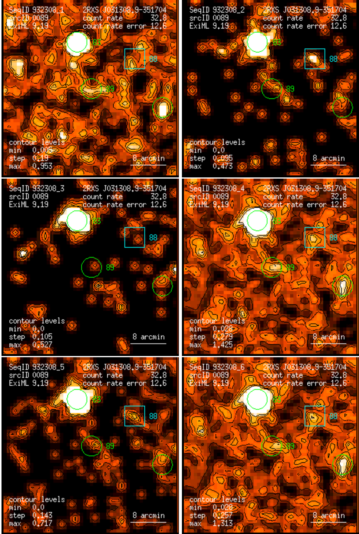
Figure 89: RASS 932308: detection 0089: band rate images, Gaussian filter: (1) PSPC channels 11 – 41, (2) 52 – 90, (3) 91 – 201, (4) 11 – 235, (5) 52 – 201, (6) 11 – 201. Broad band rates in counts/ks. Band rate contour levels in counts/ks/arcmin 2 .
