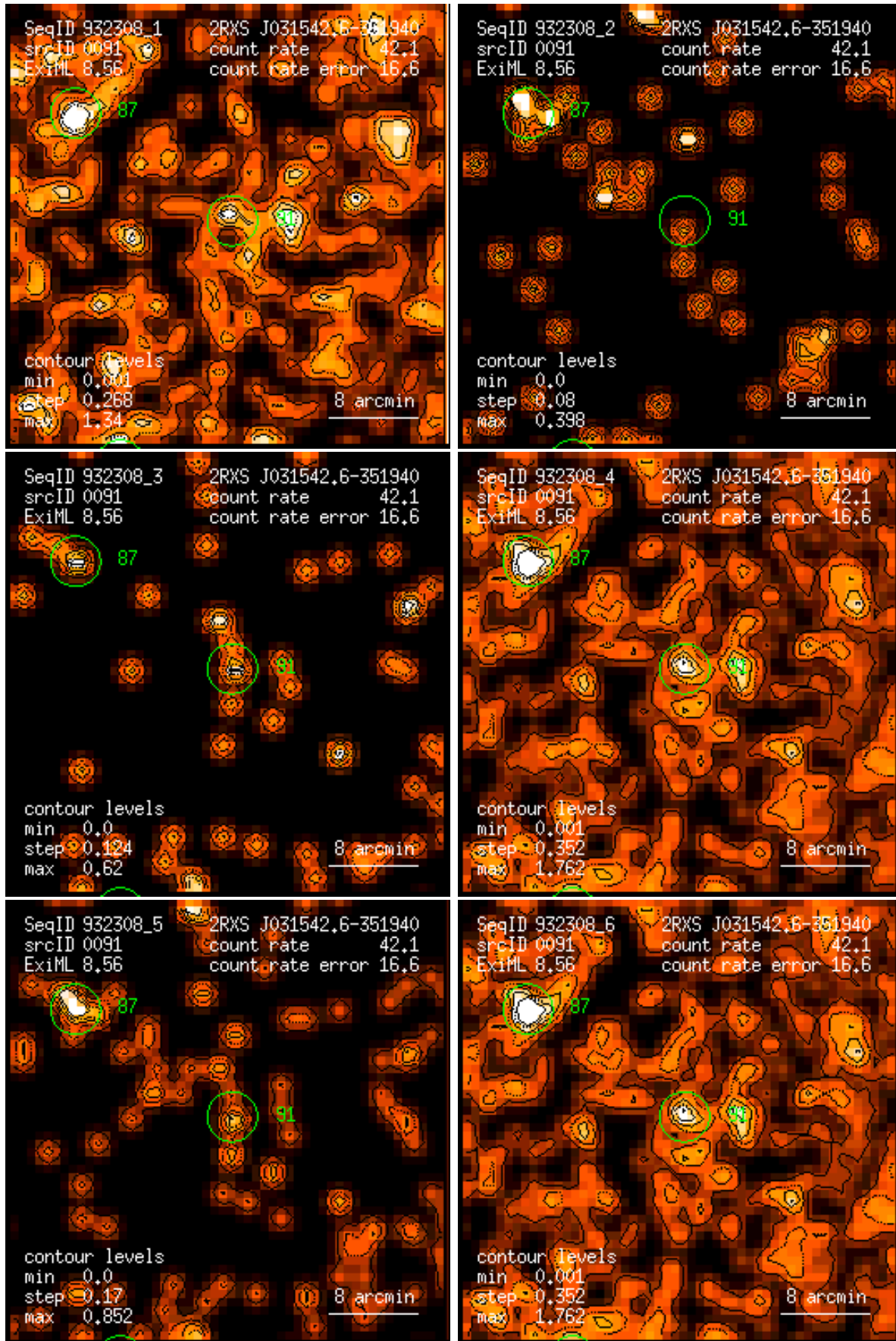
Figure 91: RASS 932308: detection 0091: band rate images, Gaussian filter: (1) PSPC channels 11 – 41, (2) 52 – 90, (3) 91 – 201, (4) 11 – 235, (5) 52 – 201, (6) 11 – 201. Broad band rates in counts/ks. Band rate contour levels in counts/ks/arcmin 2 .
