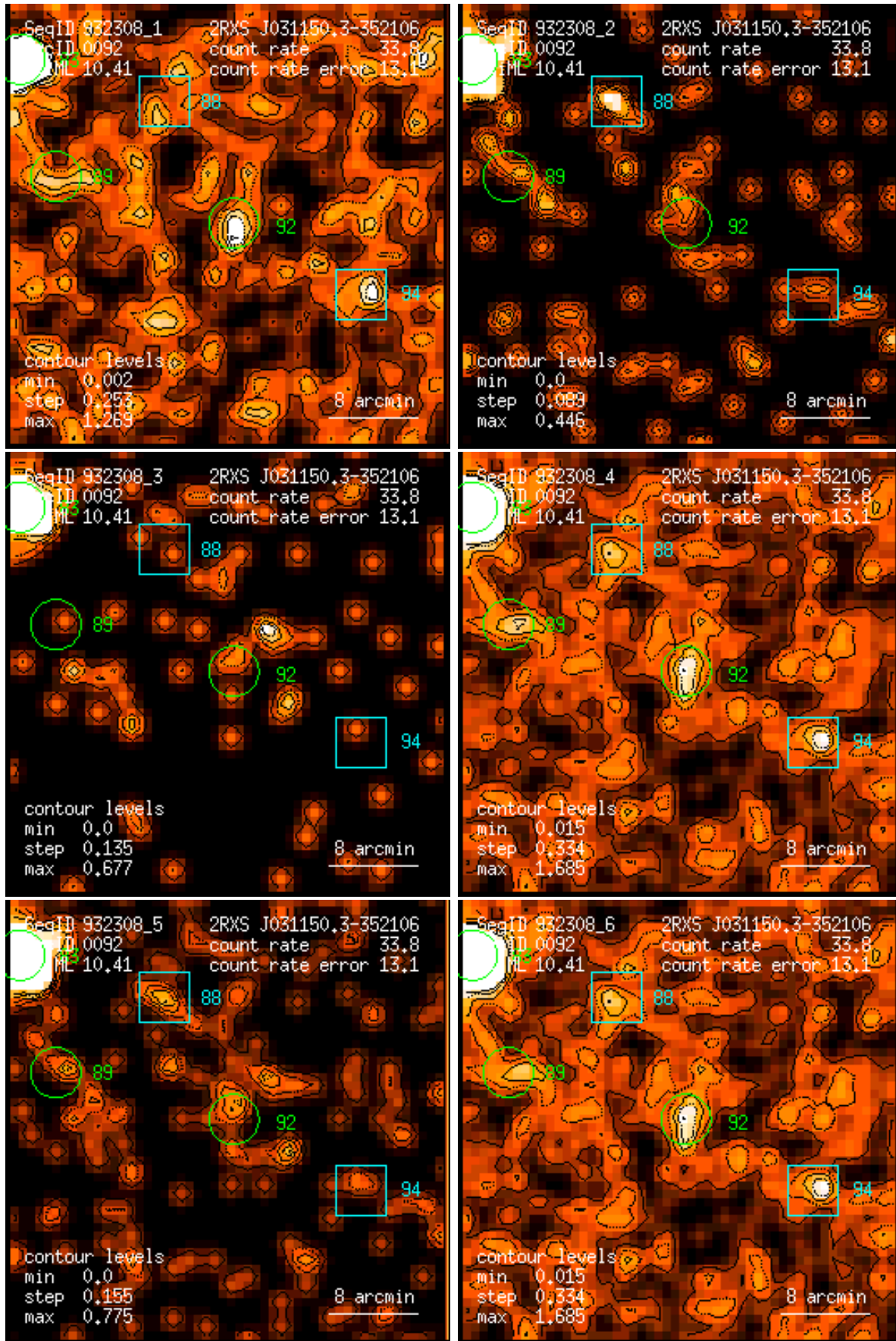
Figure 92: RASS 932308: detection 0092: band rate images, Gaussian filter: (1) PSPC channels 11 – 41, (2) 52 – 90, (3) 91 – 201, (4) 11 – 235, (5) 52 – 201, (6) 11 – 201. Broad band rates in counts/ks. Band rate contour levels in counts/ks/arcmin 2 .
