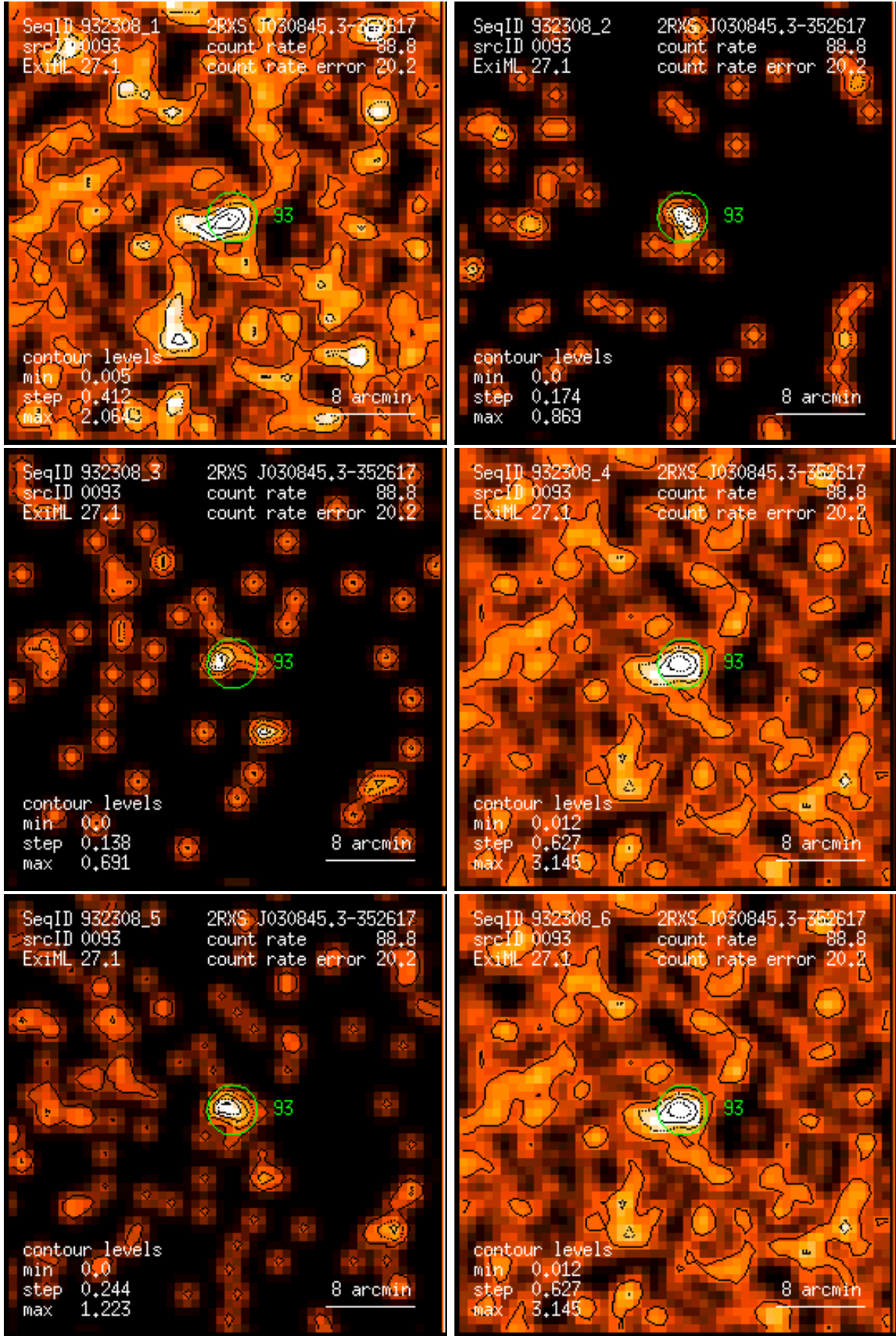
Figure 93: RASS 932308: detection 0093: band rate images, Gaussian filter: (1) PSPC channels 11 – 41, (2) 52 – 90, (3) 91 – 201, (4) 11 – 235, (5) 52 – 201, (6) 11 – 201. Broad band rates in counts/ks. Band rate contour levels in counts/ks/arcmin 2 .
