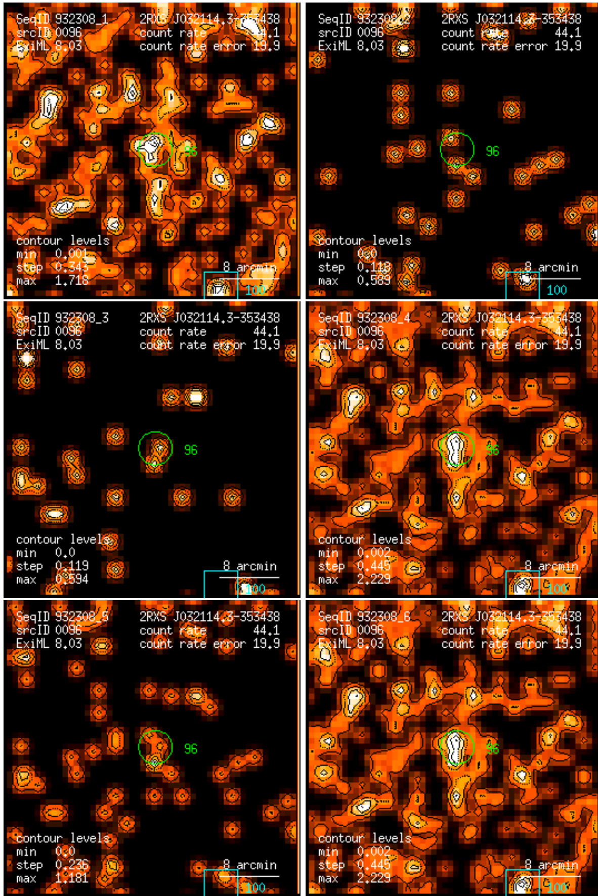
Figure 96: RASS 932308: detection 0096: band rate images, Gaussian filter: (1) PSPC channels 11 – 41, (2) 52 – 90, (3) 91 – 201, (4) 11 – 235, (5) 52 – 201, (6) 11 – 201. Broad band rates in counts/ks. Band rate contour levels in counts/ks/arcmin 2 .
