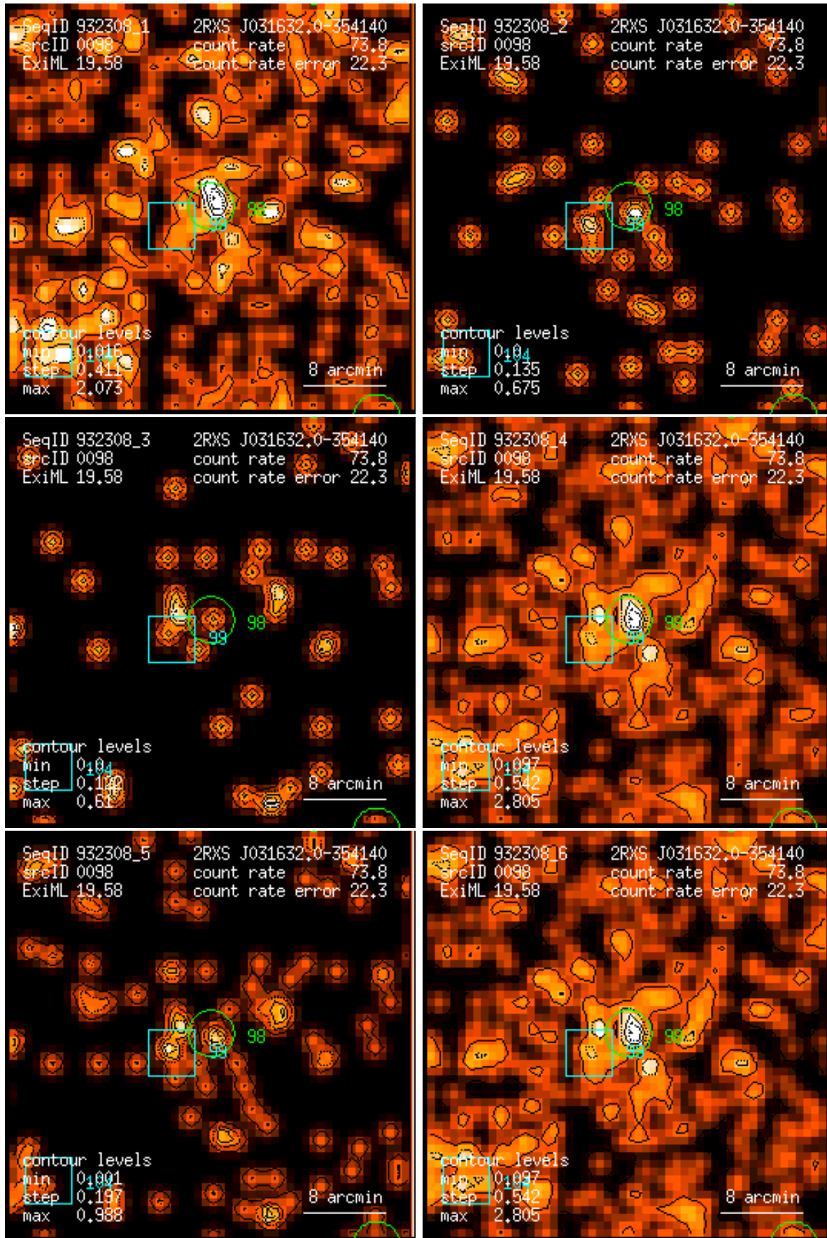
Figure 98: RASS 932308: detection 0098: band rate images, Gaussian filter: (1) PSPC channels 11 – 41, (2) 52 – 90, (3) 91 – 201, (4) 11 – 235, (5) 52 – 201, (6) 11 – 201. Broad band rates in counts/ks. Band rate contour levels in counts/ks/arcmin 2 .
