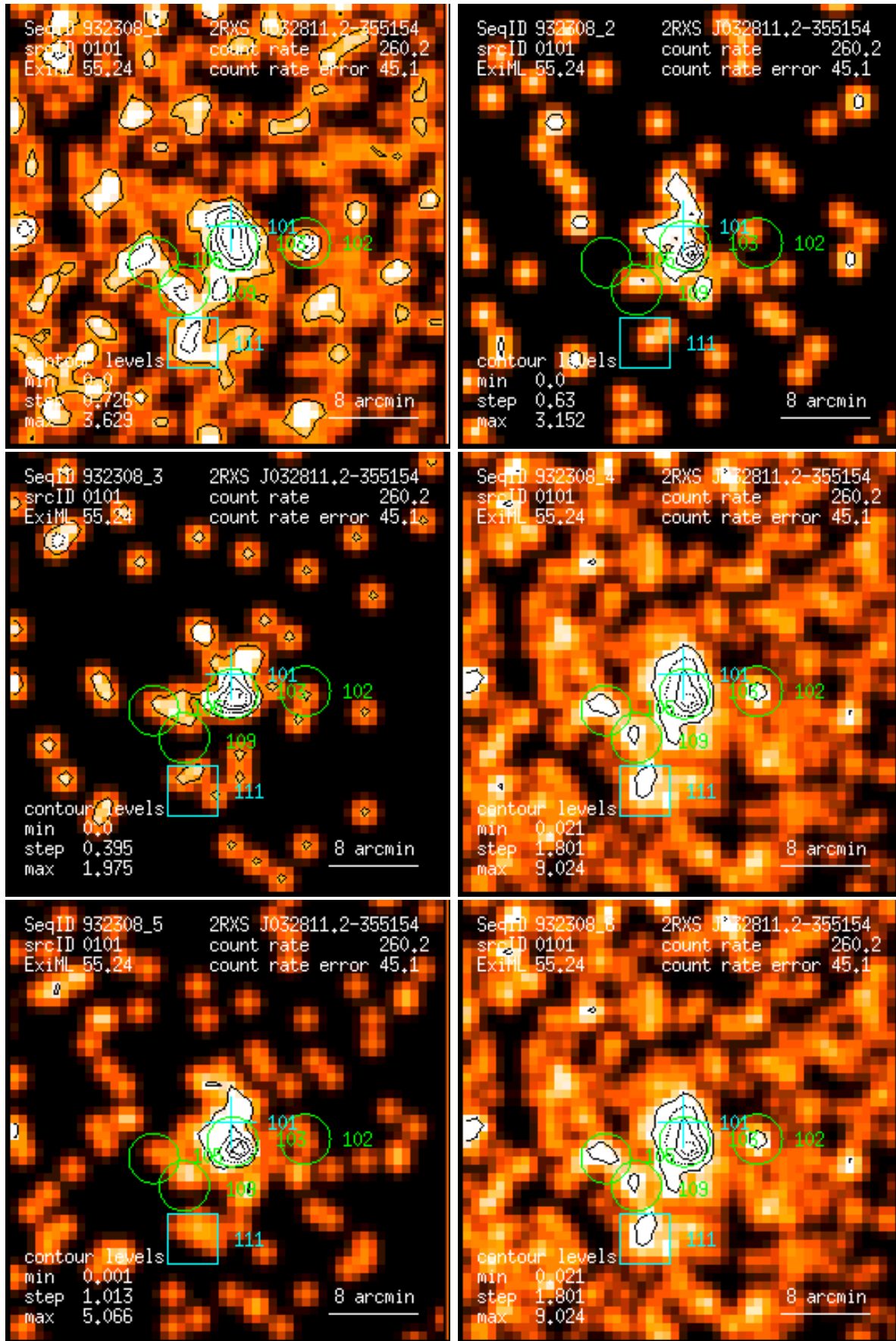
Figure 101: RASS 932308: detection 0101: band rate images, Gaussian filter: (1) PSPC channels 11 – 41, (2) 52 – 90, (3) 91 – 201, (4) 11 – 235, (5) 52 – 201, (6) 11 – 201. Broad band rates in counts/ks. Band rate contour levels in counts/ks/arcmin 2 .
