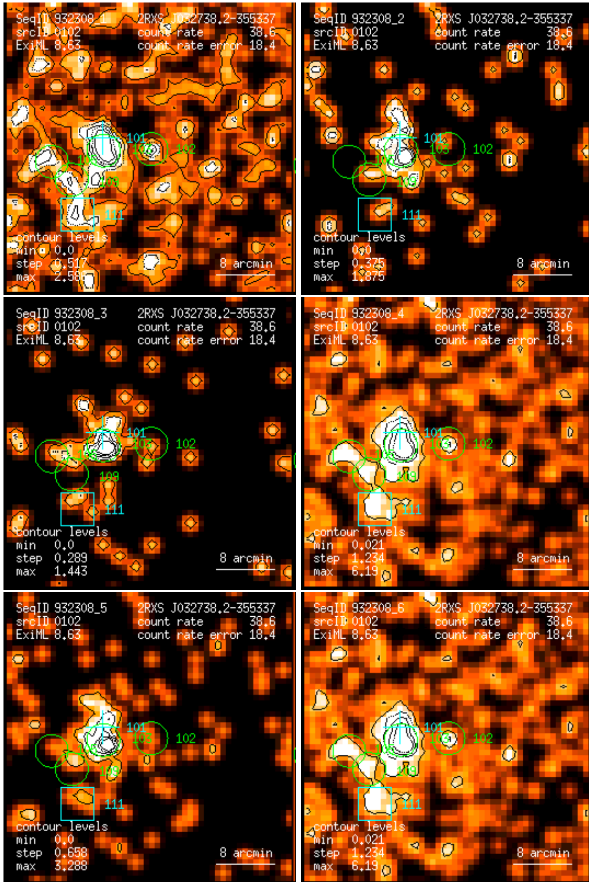
Figure 102: RASS 932308: detection 0102: band rate images, Gaussian filter: (1) PSPC channels 11 – 41, (2) 52 – 90, (3) 91 – 201, (4) 11 – 235, (5) 52 – 201, (6) 11 – 201. Broad band rates in counts/ks. Band rate contour levels in counts/ks/arcmin 2 .
