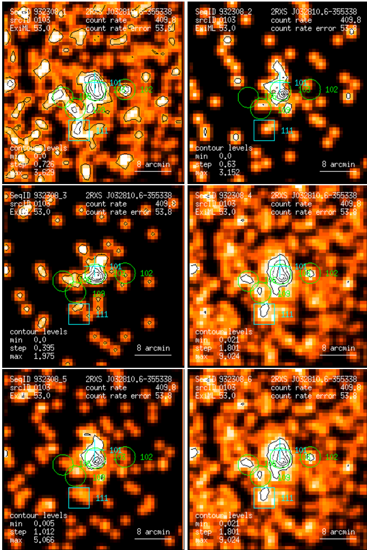
Figure 103: RASS 932308: detection 0103: band rate images, Gaussian filter: (1) PSPC channels 11 – 41, (2) 52 – 90, (3) 91 – 201, (4) 11 – 235, (5) 52 – 201, (6) 11 – 201. Broad band rates in counts/ks. Band rate contour levels in counts/ks/arcmin 2 .
