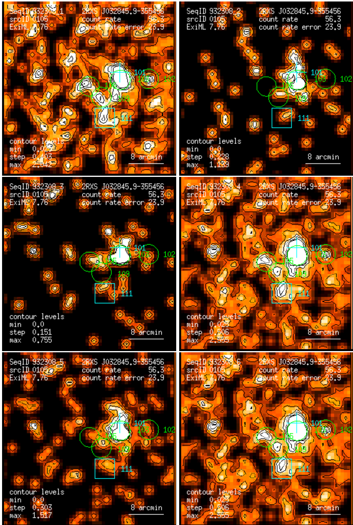
Figure 105: RASS 932308: detection 0105: band rate images, Gaussian filter: (1) PSPC channels 11 – 41, (2) 52 – 90, (3) 91 – 201, (4) 11 – 235, (5) 52 – 201, (6) 11 – 201. Broad band rates in counts/ks. Band rate contour levels in counts/ks/arcmin 2 .
