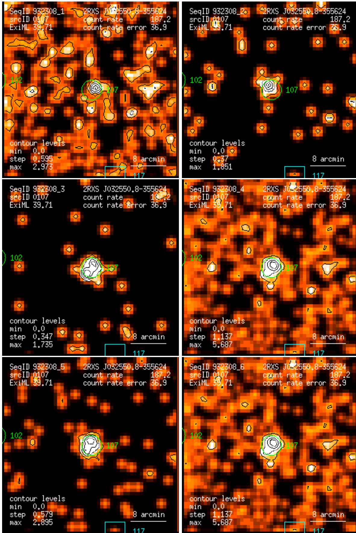
Figure 107: RASS 932308: detection 0107: band rate images, Gaussian filter: (1) PSPC channels 11 – 41, (2) 52 – 90, (3) 91 – 201, (4) 11 – 235, (5) 52 – 201, (6) 11 – 201. Broad band rates in counts/ks. Band rate contour levels in counts/ks/arcmin 2 .
