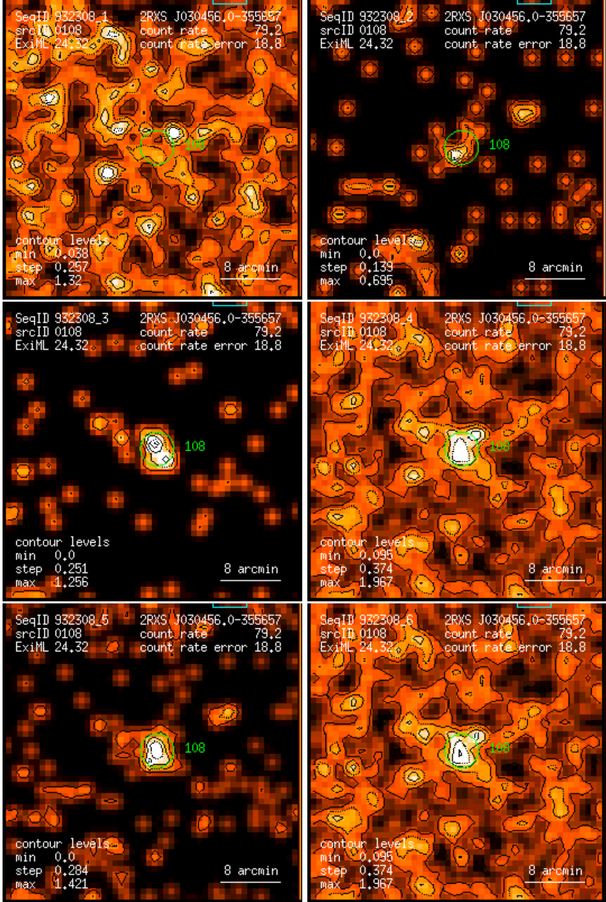
Figure 108: RASS 932308: detection 0108: band rate images, Gaussian filter: (1) PSPC channels 11 – 41, (2) 52 – 90, (3) 91 – 201, (4) 11 – 235, (5) 52 – 201, (6) 11 – 201. Broad band rates in counts/ks. Band rate contour levels in counts/ks/arcmin 2 .
