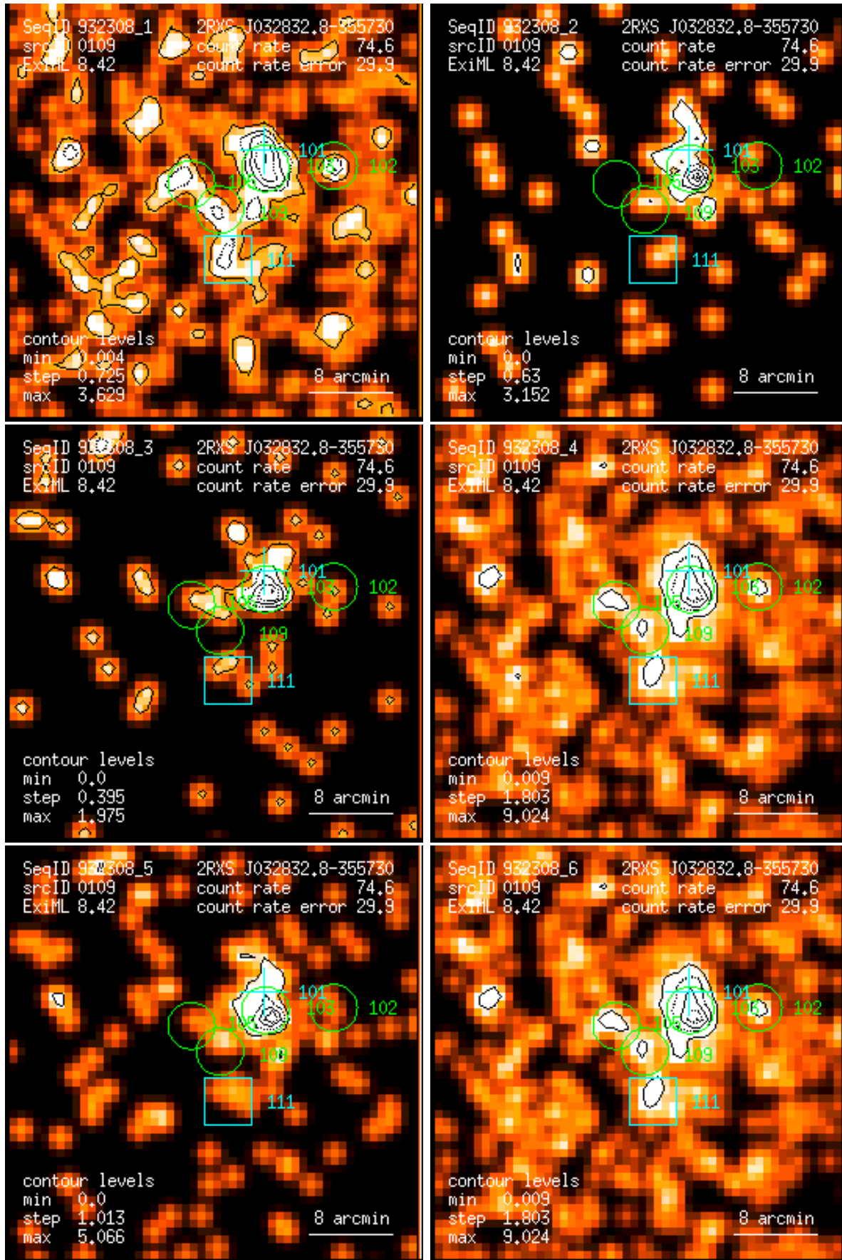
Figure 109: RASS 932308: detection 0109: band rate images, Gaussian filter: (1) PSPC channels 11 – 41, (2) 52 – 90, (3) 91 – 201, (4) 11 – 235, (5) 52 – 201, (6) 11 – 201. Broad band rates in counts/ks. Band rate contour levels in counts/ks/arcmin 2 .
