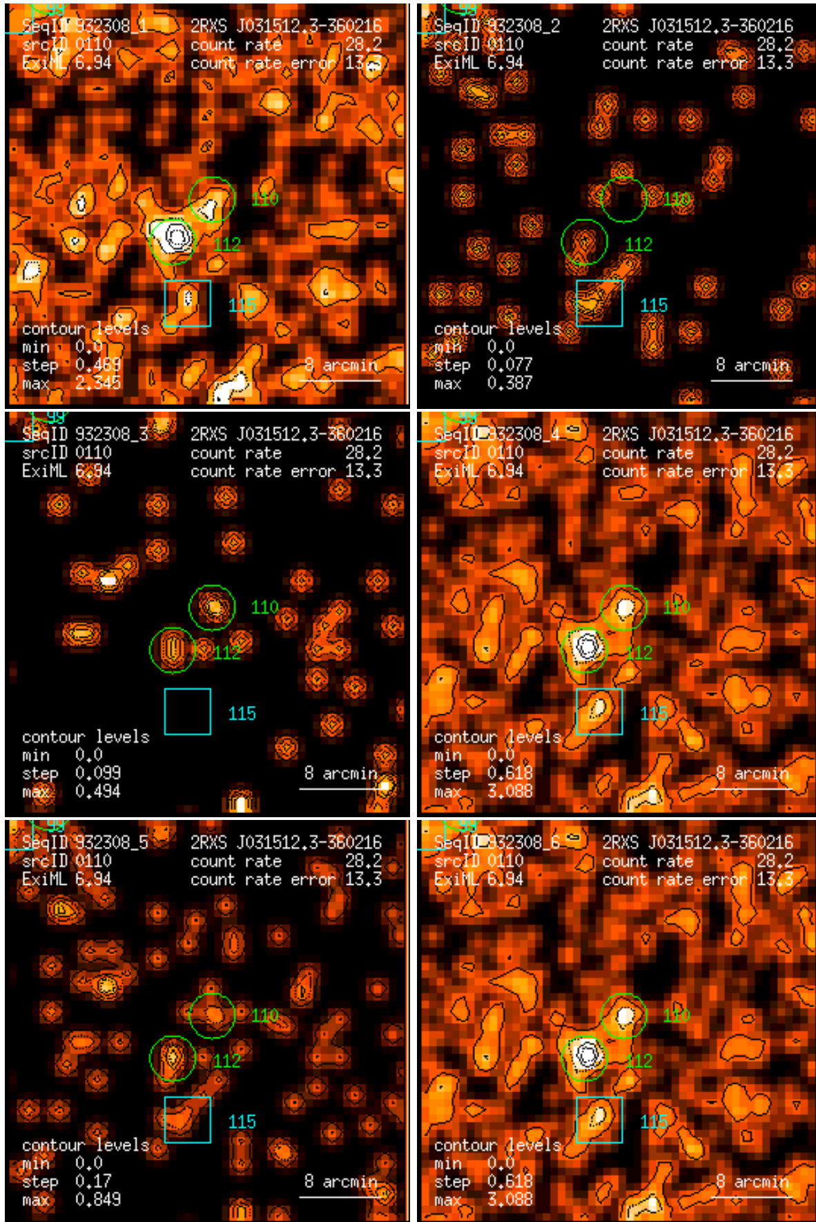
Figure 110: RASS 932308: detection 0110: band rate images, Gaussian filter: (1) PSPC channels 11 – 41, (2) 52 – 90, (3) 91 – 201, (4) 11 – 235, (5) 52 – 201, (6) 11 – 201. Broad band rates in counts/ks. Band rate contour levels in counts/ks/arcmin 2 .
