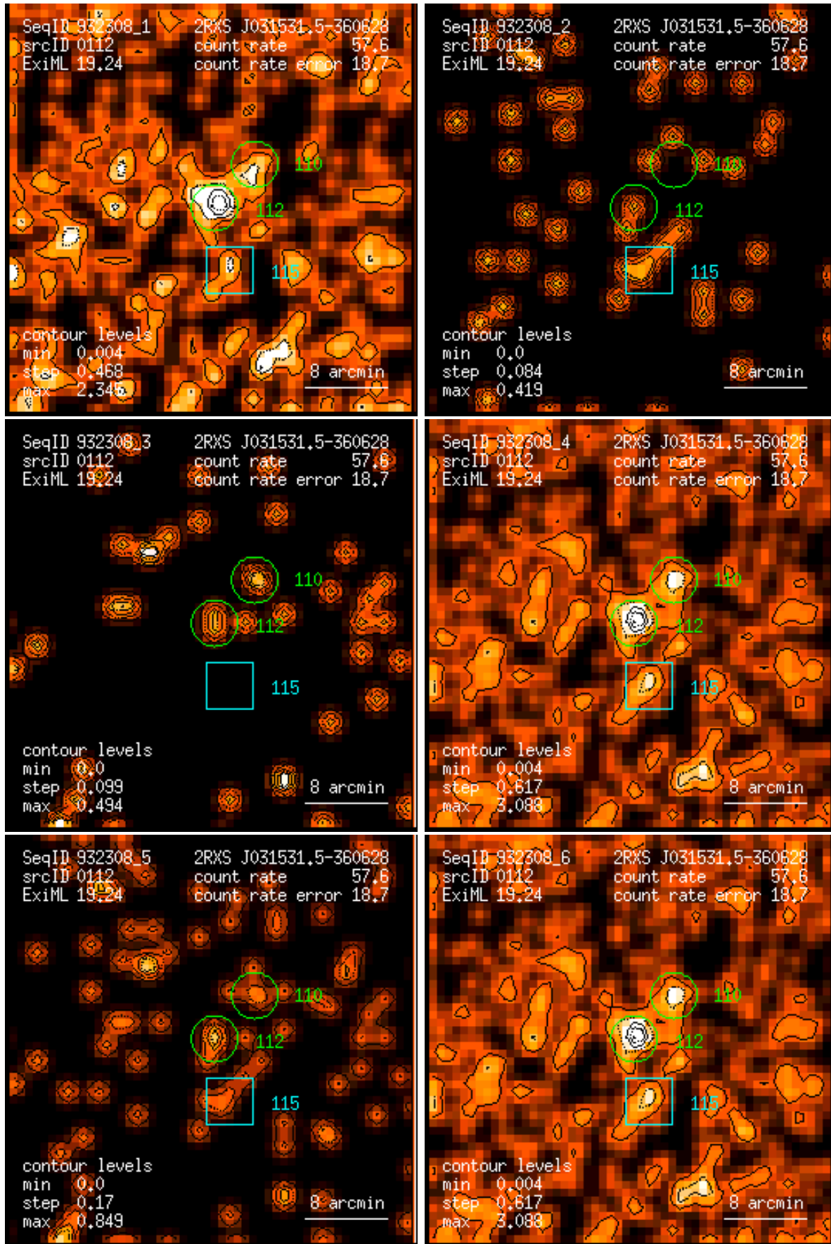
Figure 112: RASS 932308: detection 0112: band rate images, Gaussian filter: (1) PSPC channels 11 – 41, (2) 52 – 90, (3) 91 – 201, (4) 11 – 235, (5) 52 – 201, (6) 11 – 201. Broad band rates in counts/ks. Band rate contour levels in counts/ks/arcmin 2 .
