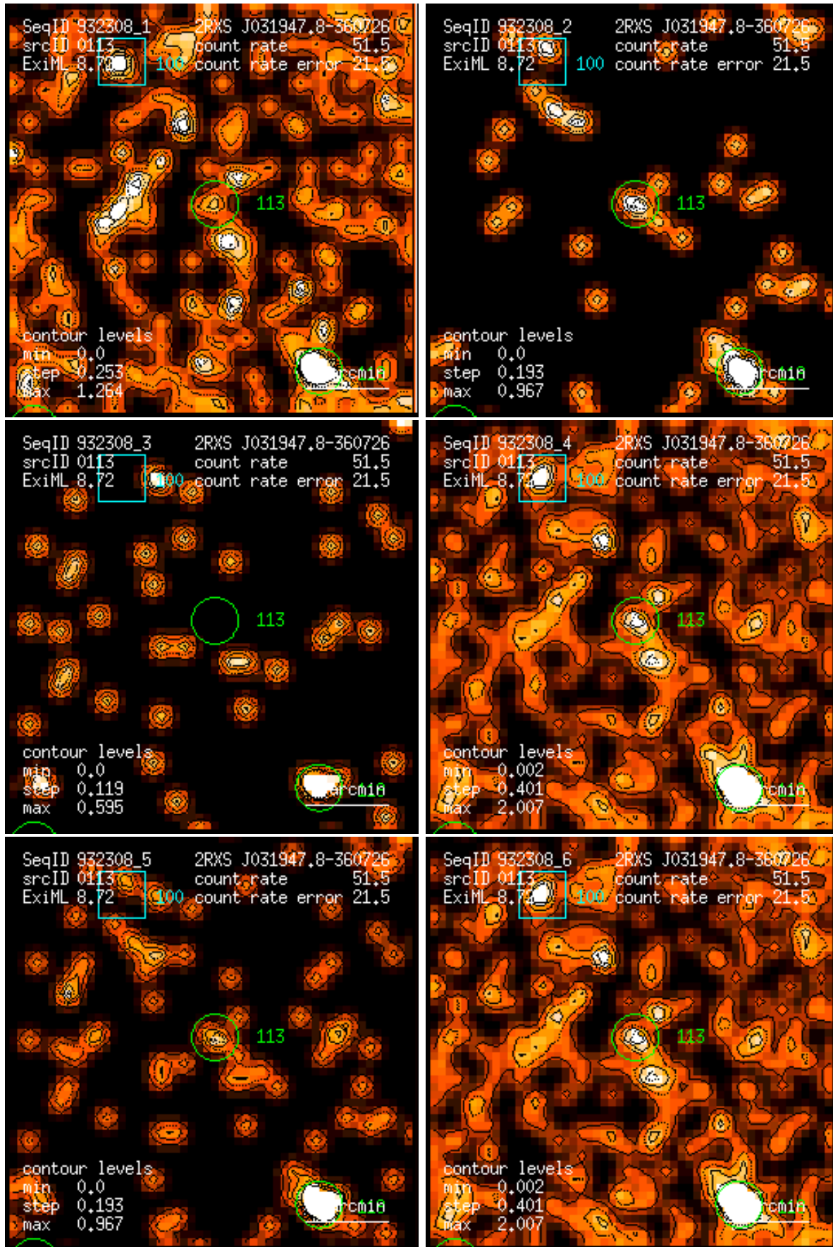
Figure 113: RASS 932308: detection 0113: band rate images, Gaussian filter: (1) PSPC channels 11 – 41, (2) 52 – 90, (3) 91 – 201, (4) 11 – 235, (5) 52 – 201, (6) 11 – 201. Broad band rates in counts/ks. Band rate contour levels in counts/ks/arcmin 2 .
