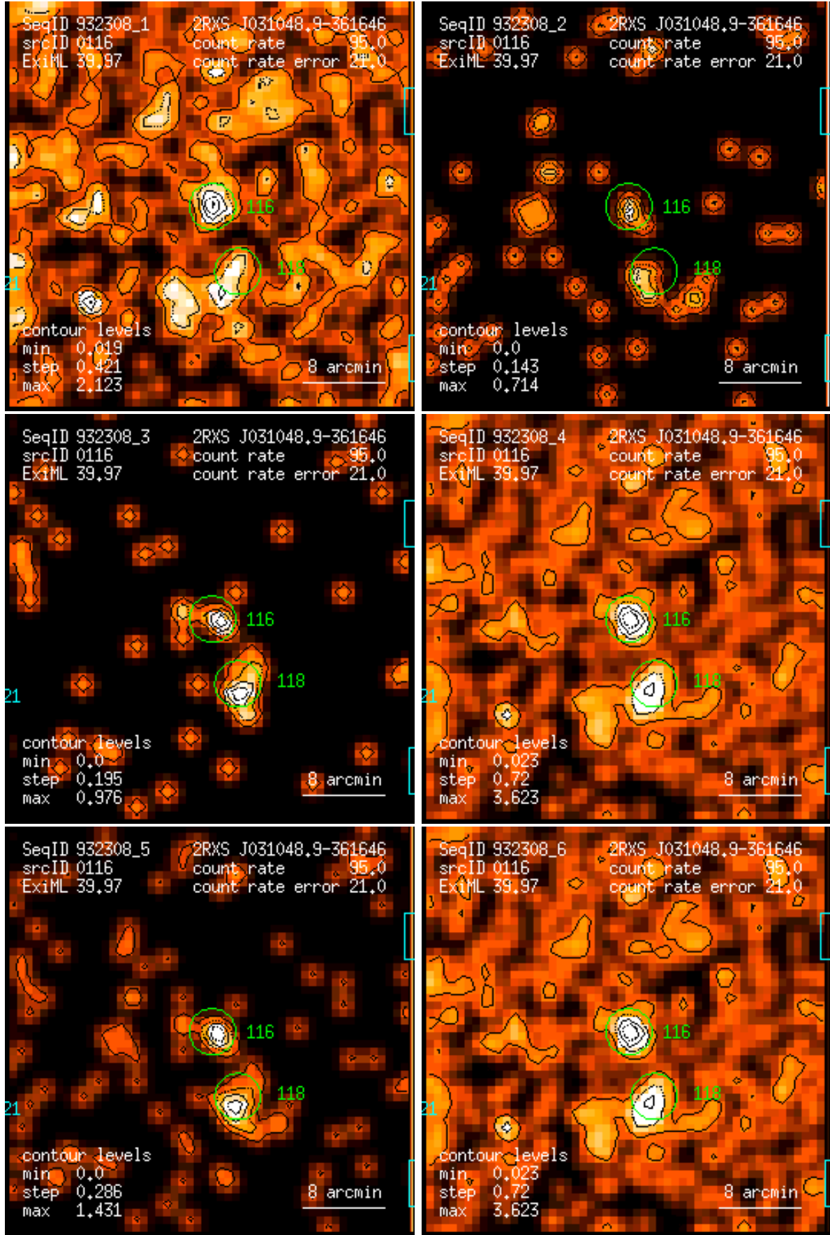
Figure 116: RASS 932308: detection 0116: band rate images, Gaussian filter: (1) PSPC channels 11 – 41, (2) 52 – 90, (3) 91 – 201, (4) 11 – 235, (5) 52 – 201, (6) 11 – 201. Broad band rates in counts/ks. Band rate contour levels in counts/ks/arcmin 2 .
