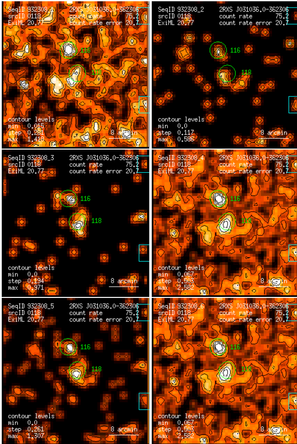
Figure 118: RASS 932308: detection 0118: band rate images, Gaussian filter: (1) PSPC channels 11 – 41, (2) 52 – 90, (3) 91 – 201, (4) 11 – 235, (5) 52 – 201, (6) 11 – 201. Broad band rates in counts/ks. Band rate contour levels in counts/ks/arcmin 2 .
