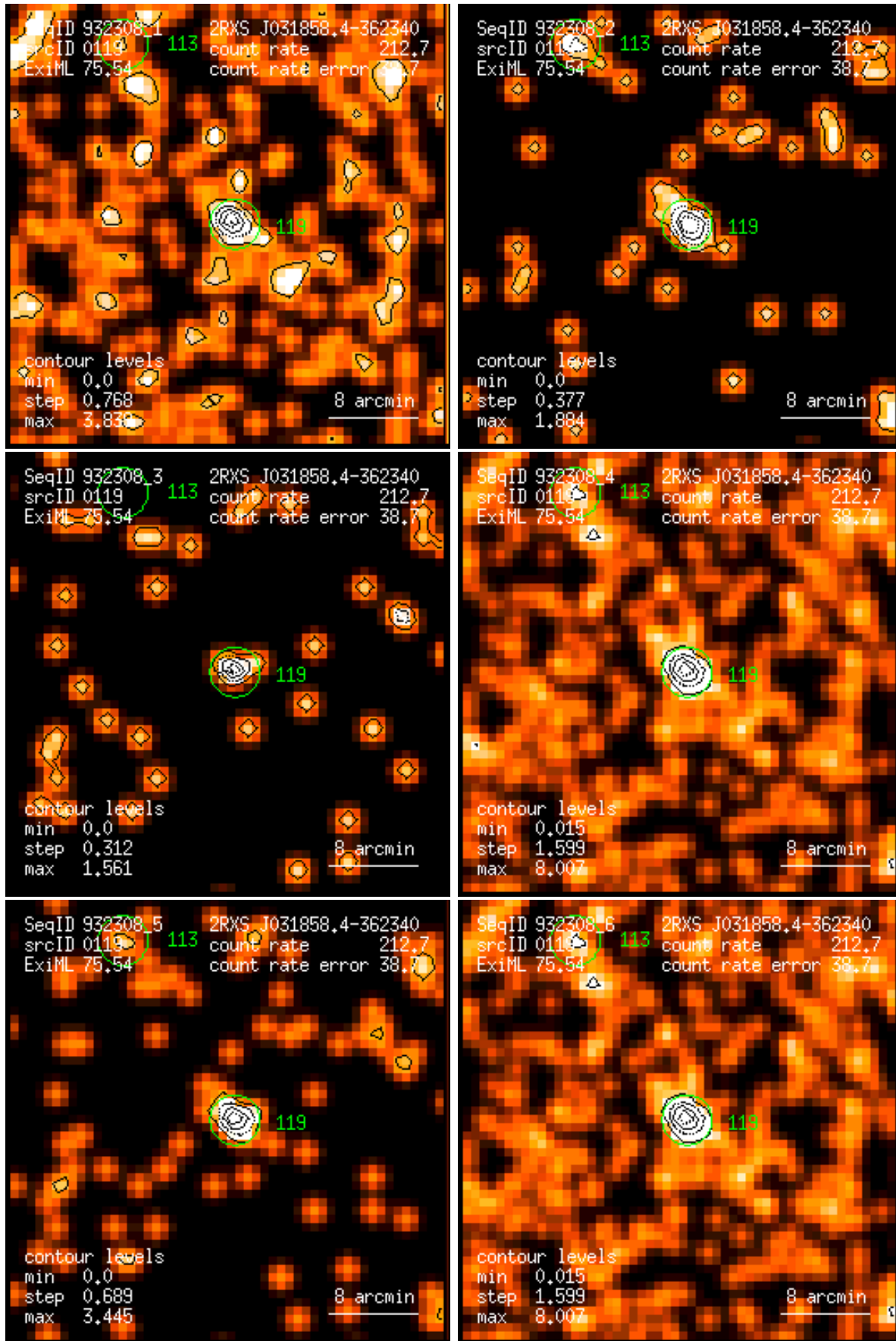
Figure 119: RASS 932308: detection 0119: band rate images, Gaussian filter: (1) PSPC channels 11 – 41, (2) 52 – 90, (3) 91 – 201, (4) 11 – 235, (5) 52 – 201, (6) 11 – 201. Broad band rates in counts/ks. Band rate contour levels in counts/ks/arcmin 2 .
