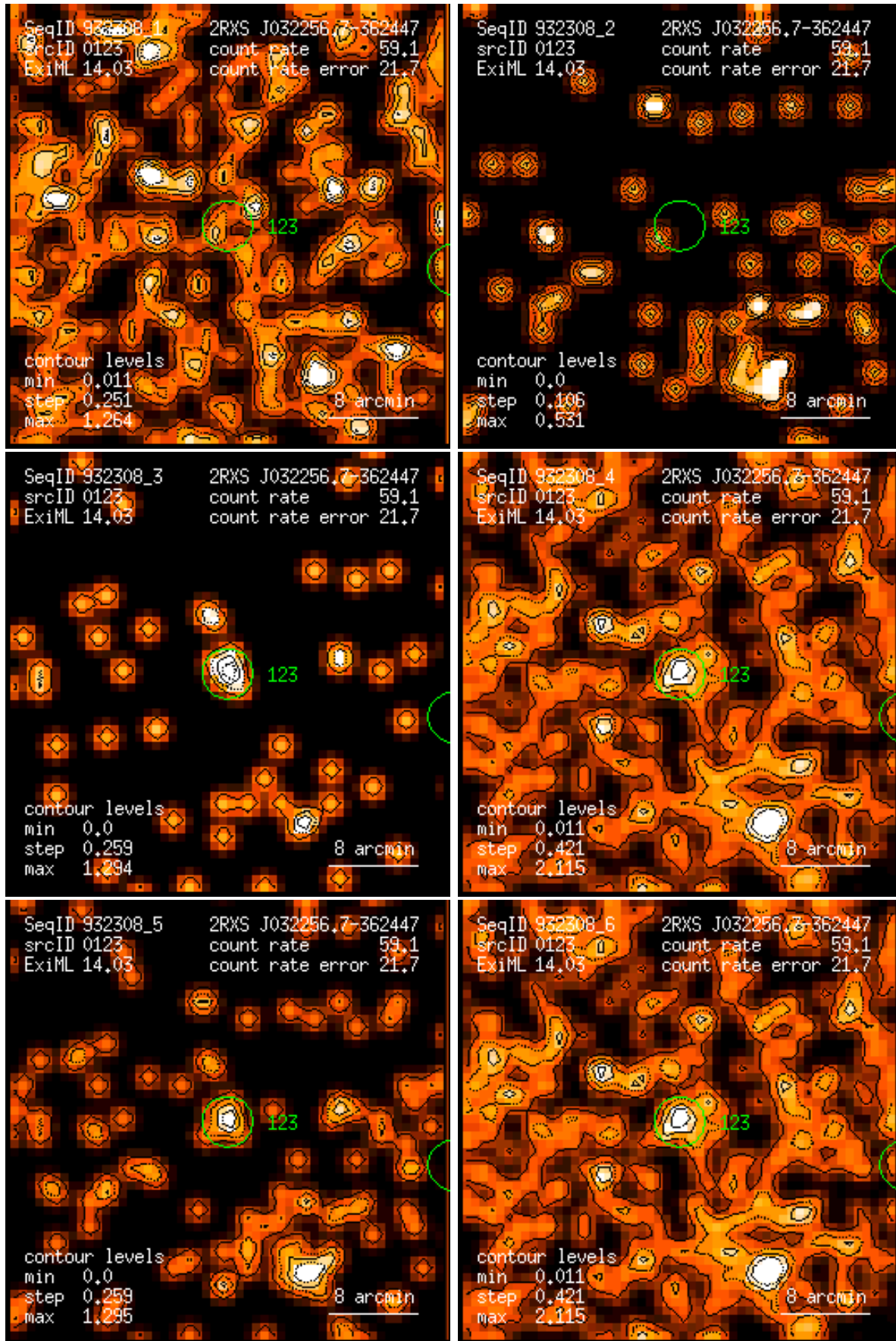
Figure 123: RASS 932308: detection 0123: band rate images, Gaussian filter: (1) PSPC channels 11 – 41, (2) 52 – 90, (3) 91 – 201, (4) 11 – 235, (5) 52 – 201, (6) 11 – 201. Broad band rates in counts/ks. Band rate contour levels in counts/ks/arcmin 2 .
