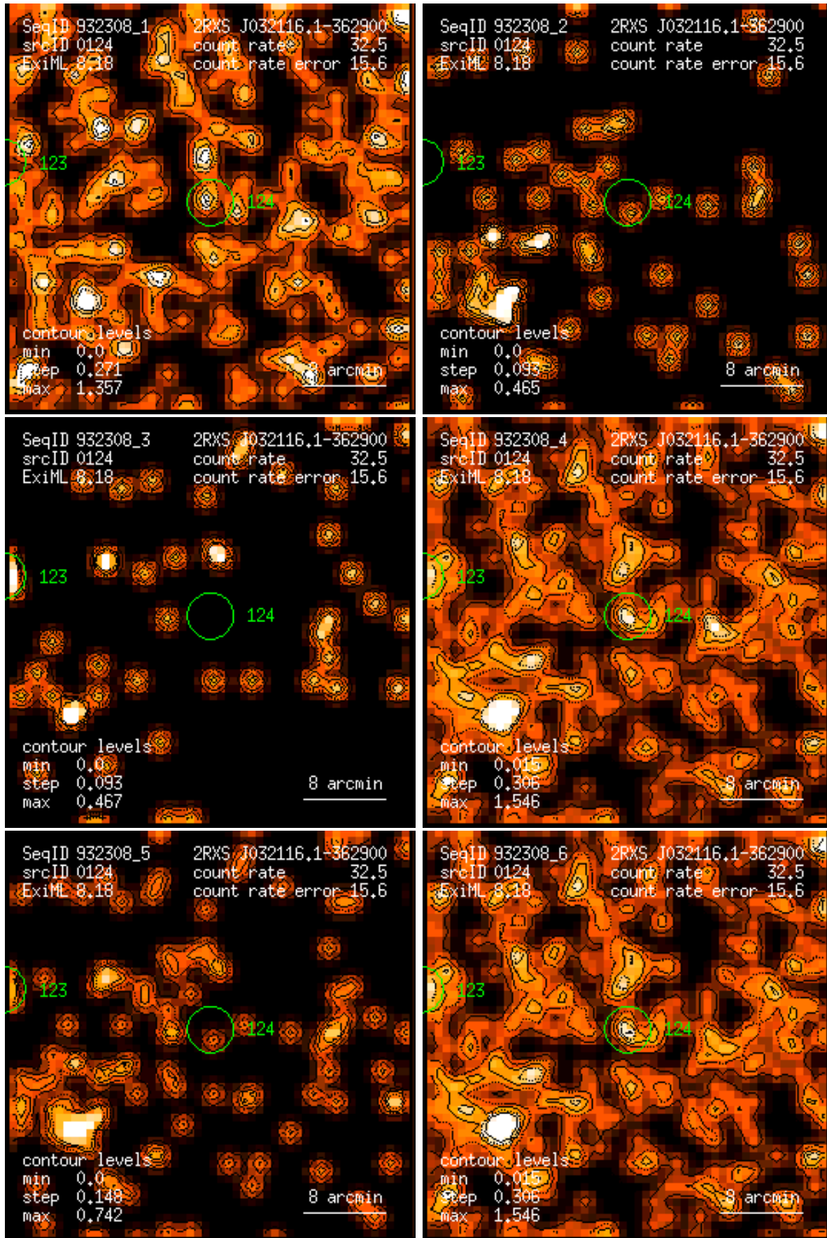
Figure 124: RASS 932308: detection 0124: band rate images, Gaussian filter: (1) PSPC channels 11 – 41, (2) 52 – 90, (3) 91 – 201, (4) 11 – 235, (5) 52 – 201, (6) 11 – 201. Broad band rates in counts/ks. Band rate contour levels in counts/ks/arcmin 2 .
