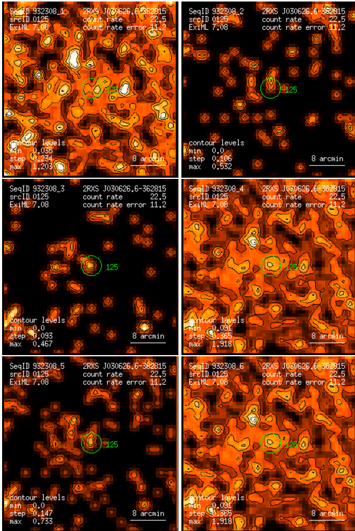
Figure 125: RASS 932308: detection 0125: band rate images, Gaussian filter: (1) PSPC channels 11 – 41, (2) 52 – 90, (3) 91 – 201, (4) 11 – 235, (5) 52 – 201, (6) 11 – 201. Broad band rates in counts/ks. Band rate contour levels in counts/ks/arcmin 2 .
