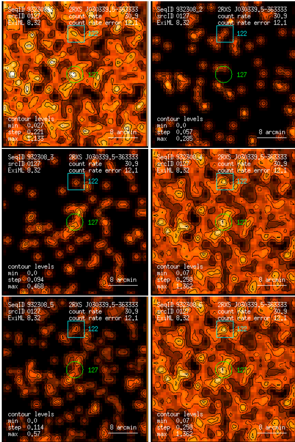
Figure 127: RASS 932308: detection 0127: band rate images, Gaussian filter: (1) PSPC channels 11 – 41, (2) 52 – 90, (3) 91 – 201, (4) 11 – 235, (5) 52 – 201, (6) 11 – 201. Broad band rates in counts/ks. Band rate contour levels in counts/ks/arcmin 2 .
