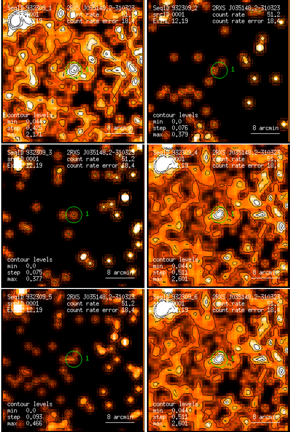
Figure 1: RASS 932309: detection 0001: band rate images, Gaussian filter: (1) PSPC channels 11 – 41, (2) 52 – 90, (3) 91 – 201, (4) 11 – 235, (5) 52 – 201, (6) 11 – 201. Broad band rates in counts/ks. Band rate contour levels in counts/ks/arcmin 2 .
