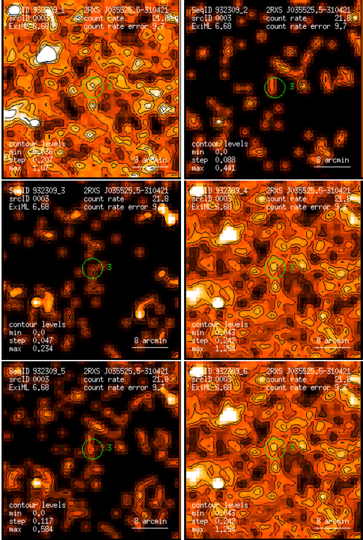
Figure 3: RASS 932309: detection 0003: band rate images, Gaussian filter: (1) PSPC channels 11 – 41, (2) 52 – 90, (3) 91 – 201, (4) 11 – 235, (5) 52 – 201, (6) 11 – 201. Broad band rates in counts/ks. Band rate contour levels in counts/ks/arcmin 2 .
