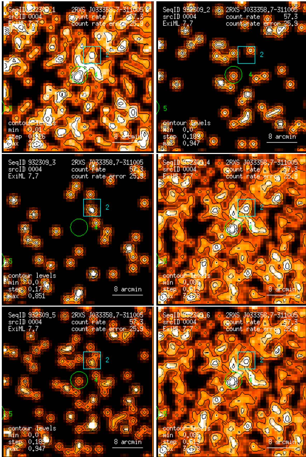
Figure 4: RASS 932309: detection 0004: band rate images, Gaussian filter: (1) PSPC channels 11 – 41, (2) 52 – 90, (3) 91 – 201, (4) 11 – 235, (5) 52 – 201, (6) 11 – 201. Broad band rates in counts/ks. Band rate contour levels in counts/ks/arcmin 2 .
