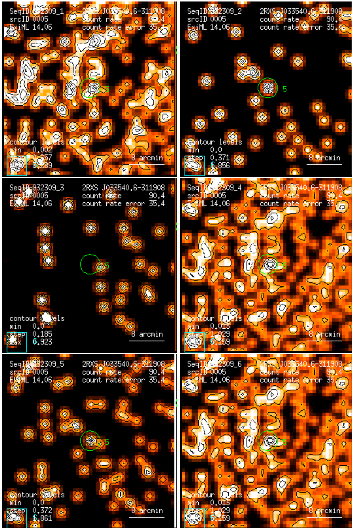
Figure 5: RASS 932309: detection 0005: band rate images, Gaussian filter: (1) PSPC channels 11 – 41, (2) 52 – 90, (3) 91 – 201, (4) 11 – 235, (5) 52 – 201, (6) 11 – 201. Broad band rates in counts/ks. Band rate contour levels in counts/ks/arcmin 2 .
