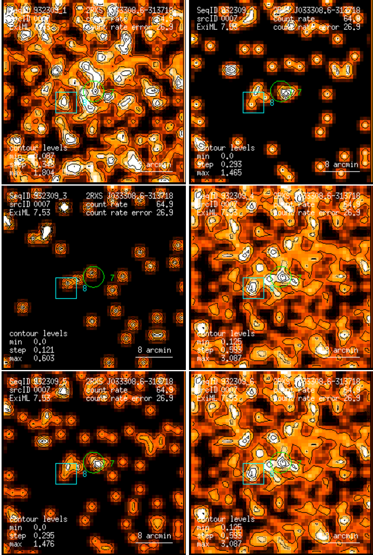
Figure 7: RASS 932309: detection 0007: band rate images, Gaussian filter: (1) PSPC channels 11 – 41, (2) 52 – 90, (3) 91 – 201, (4) 11 – 235, (5) 52 – 201, (6) 11 – 201. Broad band rates in counts/ks. Band rate contour levels in counts/ks/arcmin 2 .
