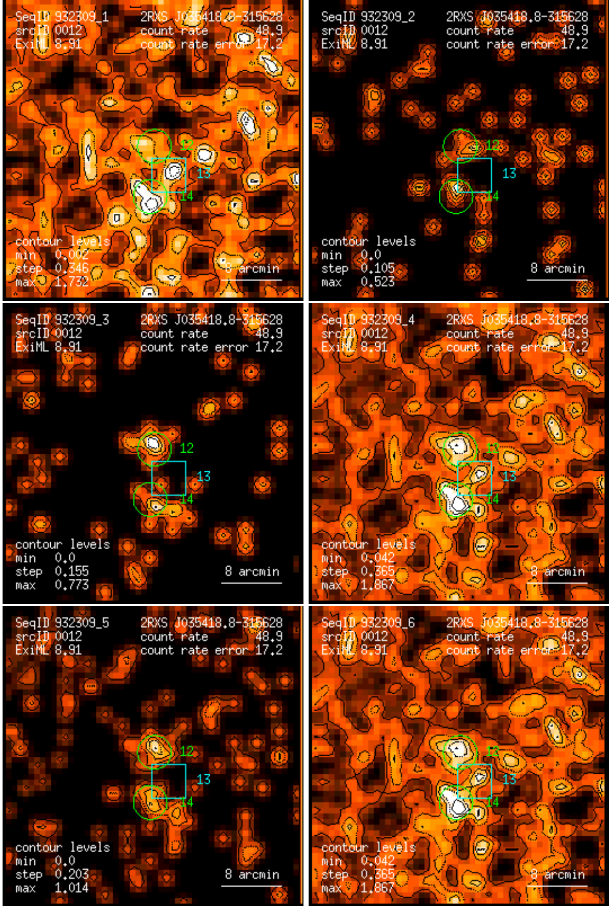
Figure 12: RASS 932309: detection 0012: band rate images, Gaussian filter: (1) PSPC channels 11 – 41, (2) 52 – 90, (3) 91 – 201, (4) 11 – 235, (5) 52 – 201, (6) 11 – 201. Broad band rates in counts/ks. Band rate contour levels in counts/ks/arcmin 2 .
