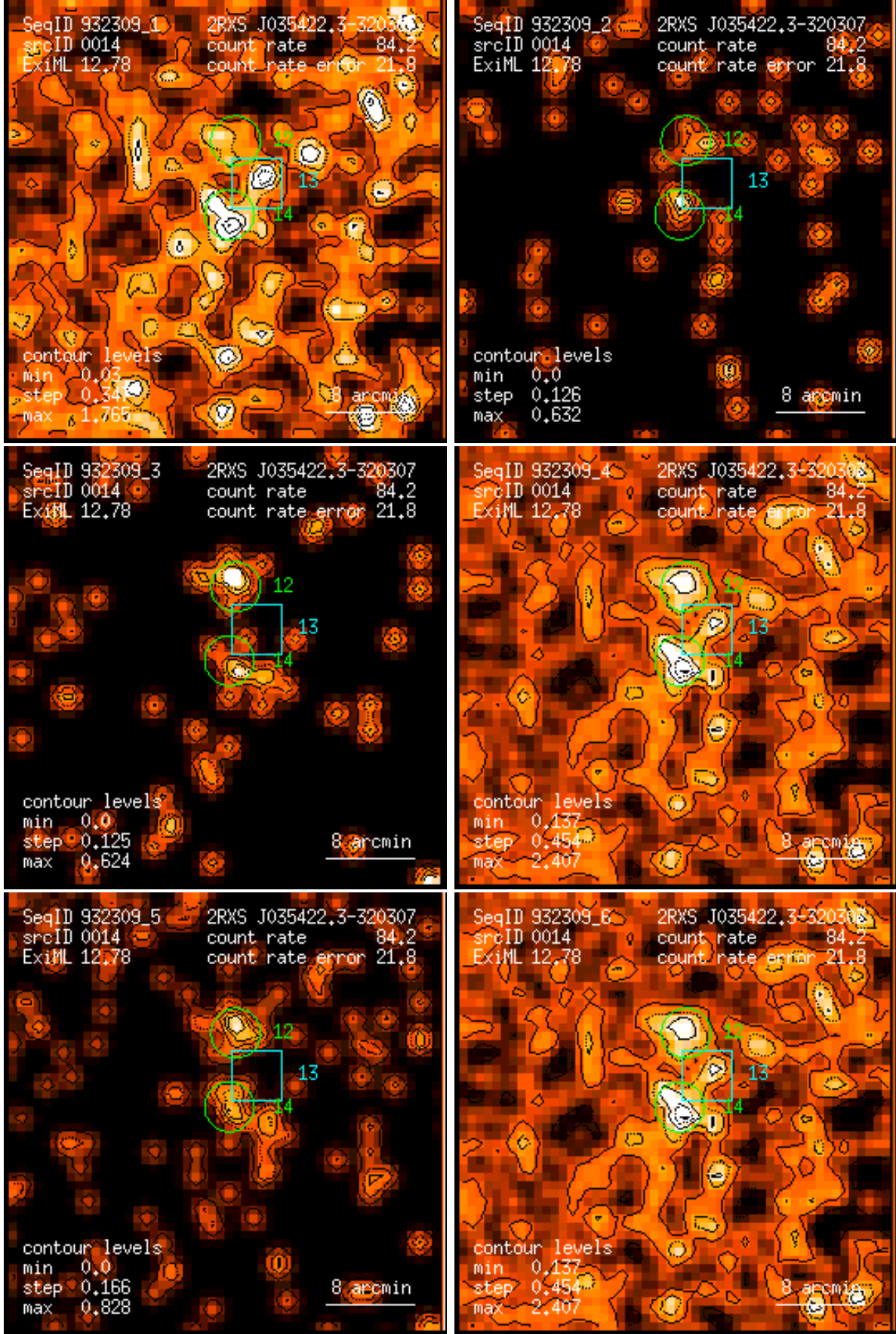
Figure 14: RASS 932309: detection 0014: band rate images, Gaussian filter: (1) PSPC channels 11 – 41, (2) 52 – 90, (3) 91 – 201, (4) 11 – 235, (5) 52 – 201, (6) 11 – 201. Broad band rates in counts/ks. Band rate contour levels in counts/ks/arcmin 2 .
