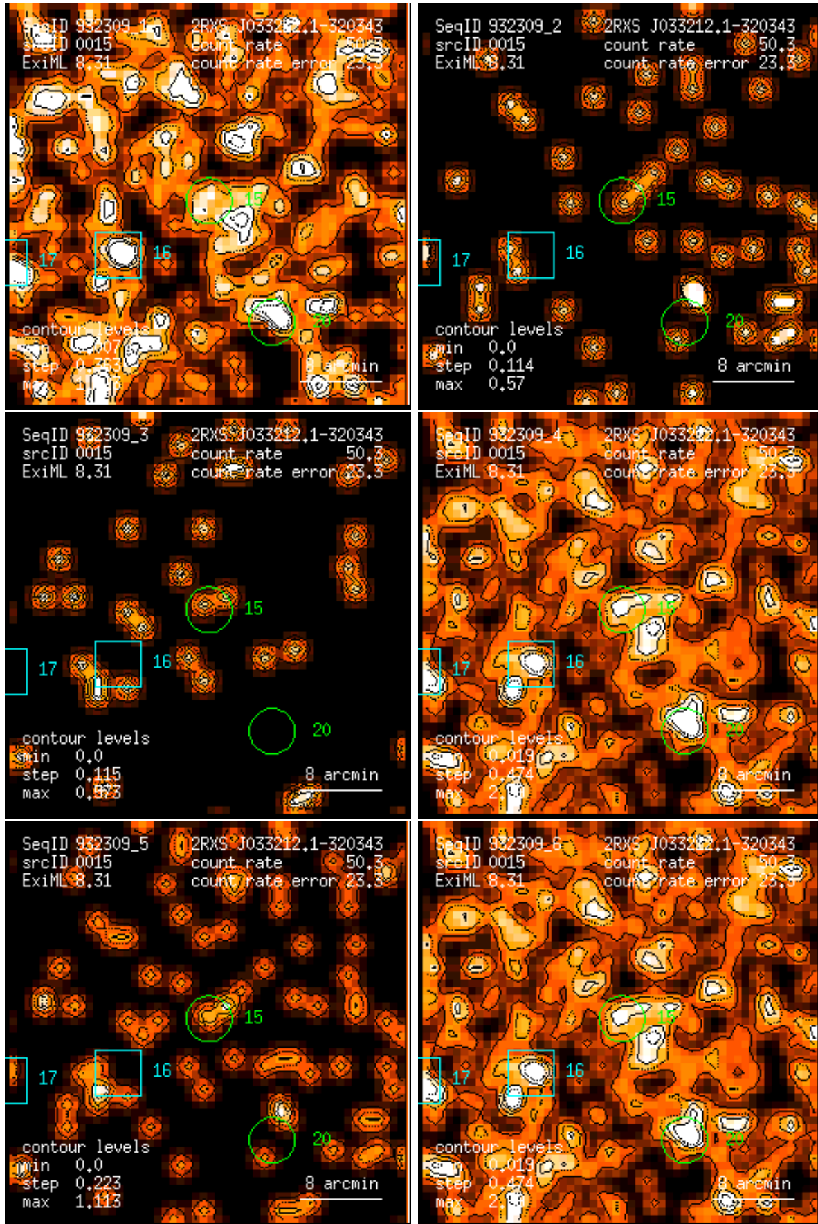
Figure 15: RASS 932309: detection 0015: band rate images, Gaussian filter: (1) PSPC channels 11 – 41, (2) 52 – 90, (3) 91 – 201, (4) 11 – 235, (5) 52 – 201, (6) 11 – 201. Broad band rates in counts/ks. Band rate contour levels in counts/ks/arcmin 2 .
