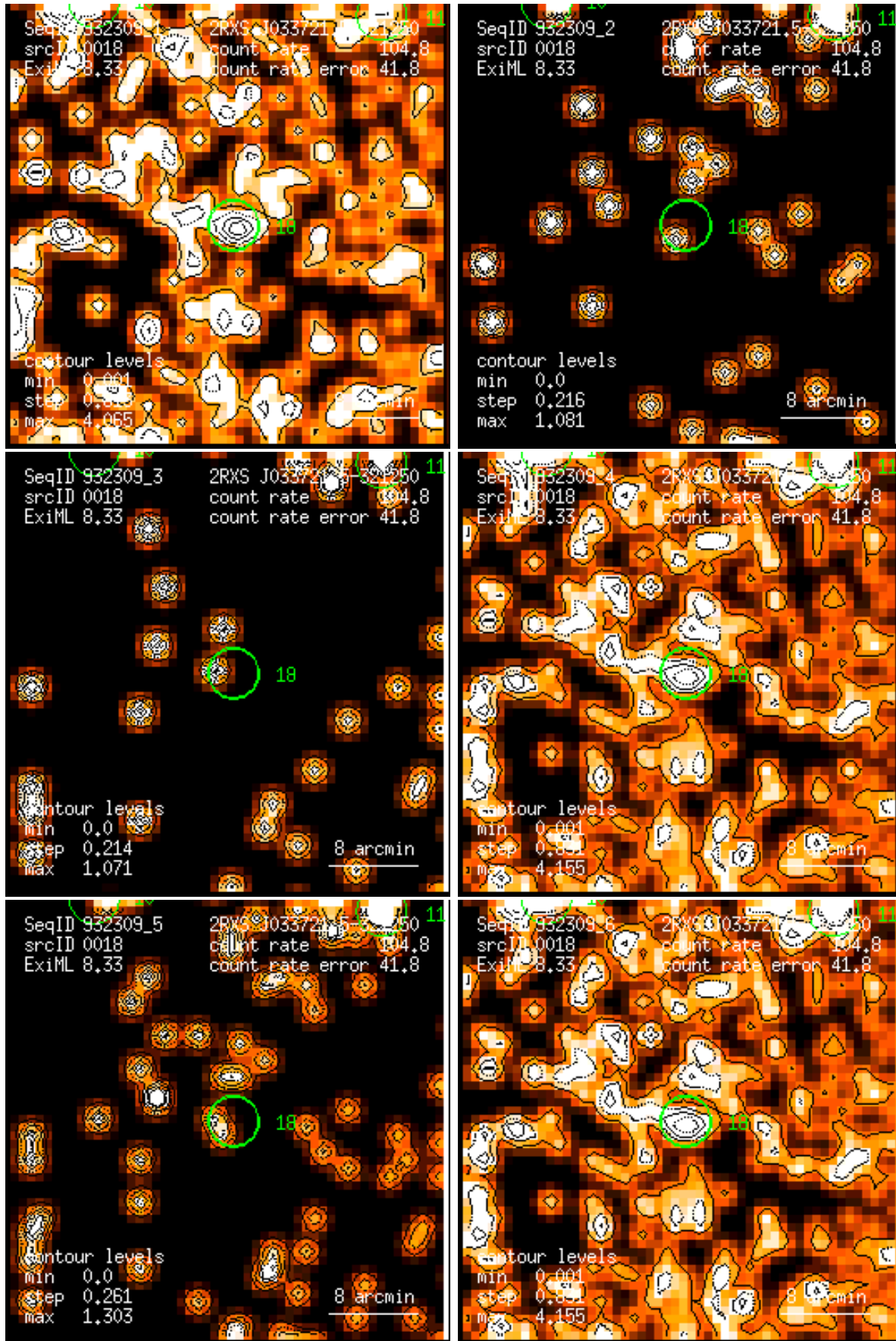
Figure 18: RASS 932309: detection 0018: band rate images, Gaussian filter: (1) PSPC channels 11 – 41, (2) 52 – 90, (3) 91 – 201, (4) 11 – 235, (5) 52 – 201, (6) 11 – 201. Broad band rates in counts/ks. Band rate contour levels in counts/ks/arcmin 2 .
