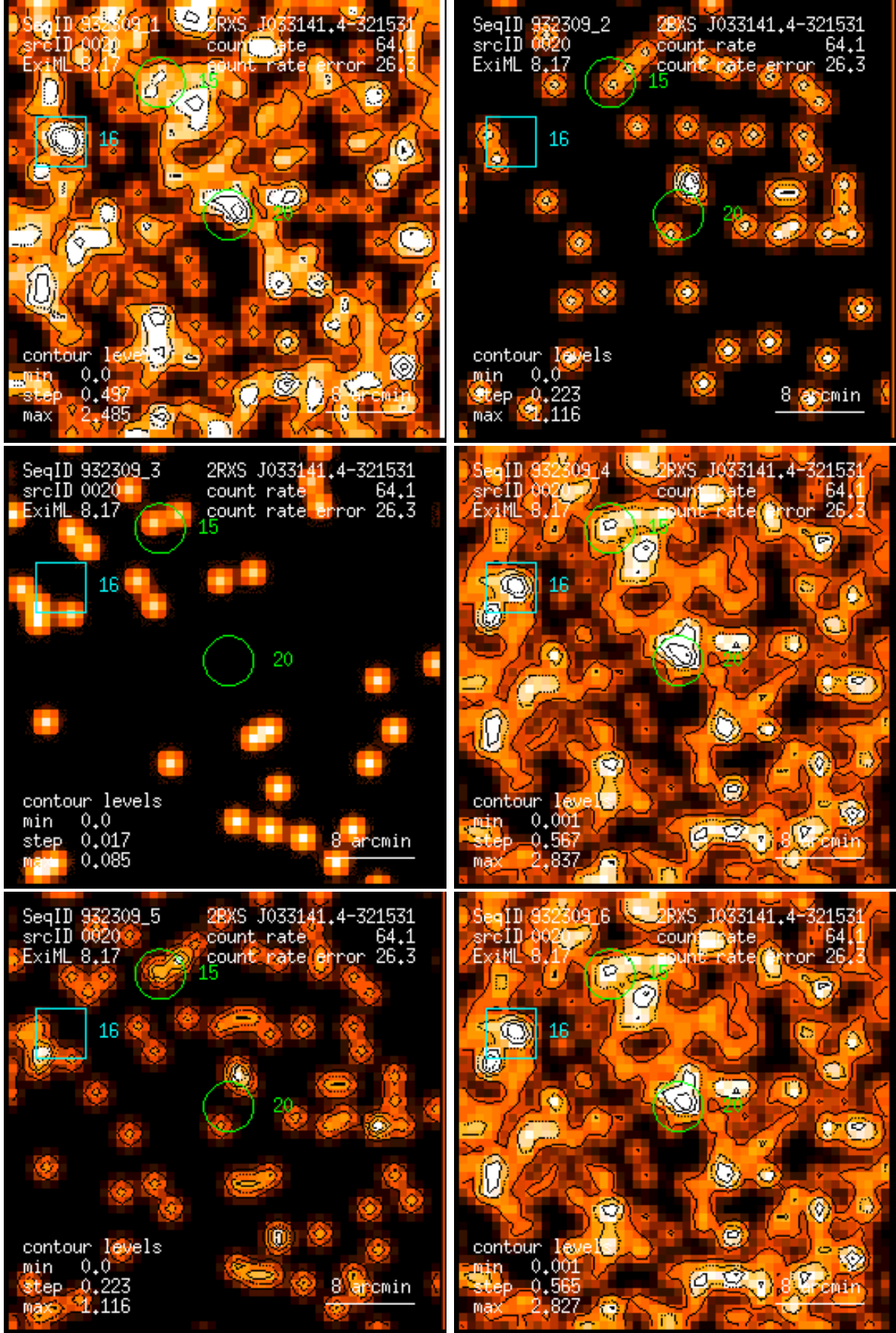
Figure 20: RASS 932309: detection 0020: band rate images, Gaussian filter: (1) PSPC channels 11 – 41, (2) 52 – 90, (3) 91 – 201, (4) 11 – 235, (5) 52 – 201, (6) 11 – 201. Broad band rates in counts/ks. Band rate contour levels in counts/ks/arcmin 2 .
