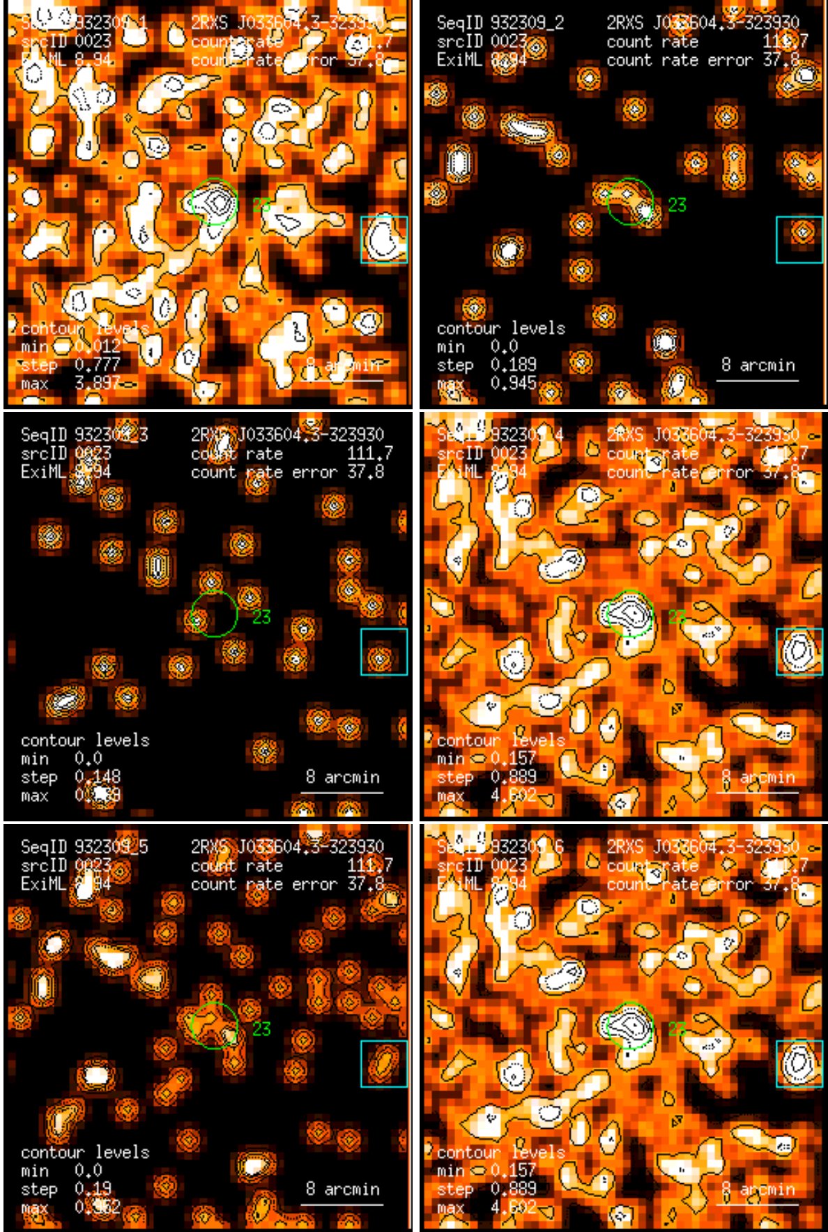
Figure 23: RASS 932309: detection 0023: band rate images, Gaussian filter: (1) PSPC channels 11 – 41, (2) 52 – 90, (3) 91 – 201, (4) 11 – 235, (5) 52 – 201, (6) 11 – 201. Broad band rates in counts/ks. Band rate contour levels in counts/ks/arcmin 2 .
