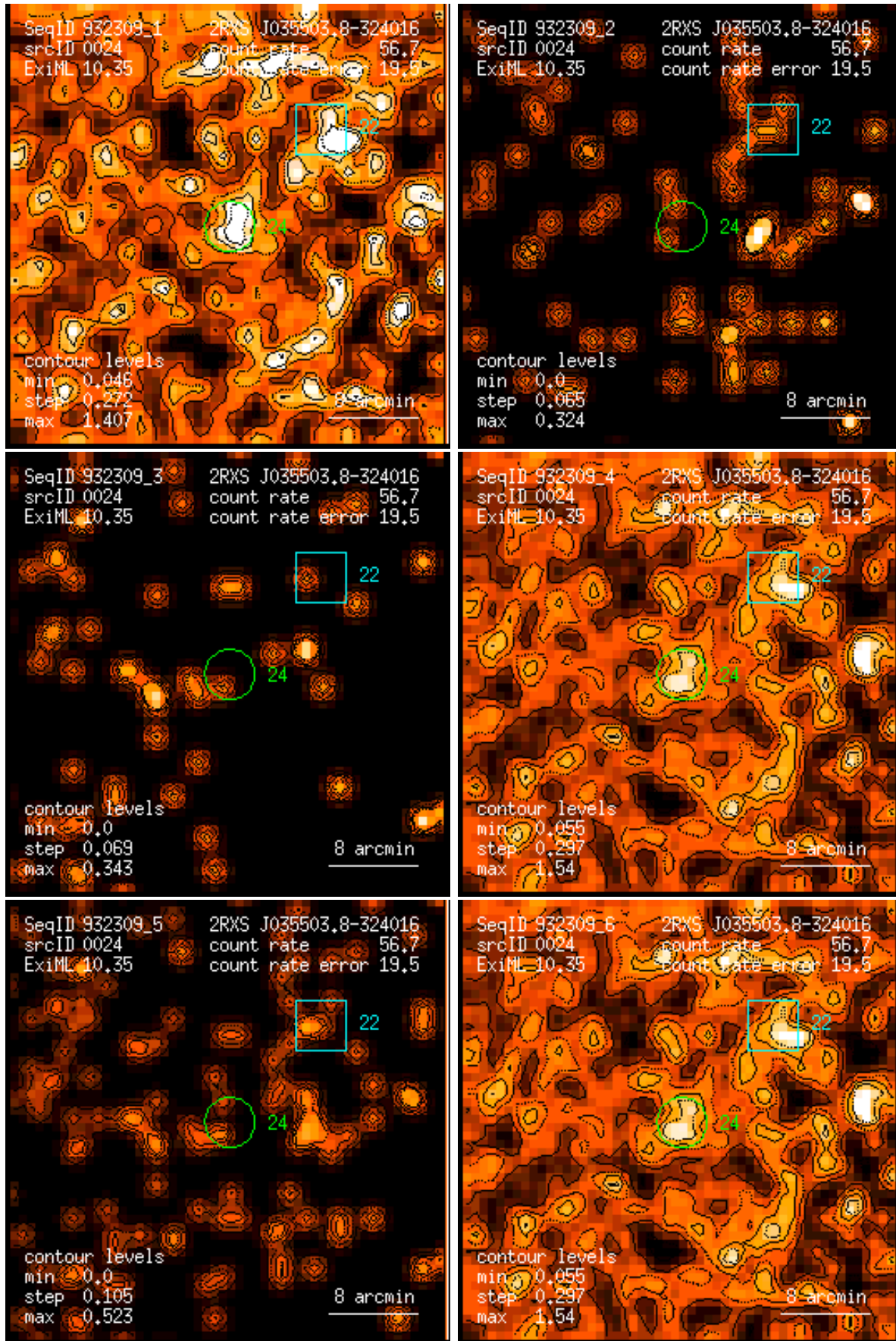
Figure 24: RASS 932309: detection 0024: band rate images, Gaussian filter: (1) PSPC channels 11 – 41, (2) 52 – 90, (3) 91 – 201, (4) 11 – 235, (5) 52 – 201, (6) 11 – 201. Broad band rates in counts/ks. Band rate contour levels in counts/ks/arcmin 2 .
