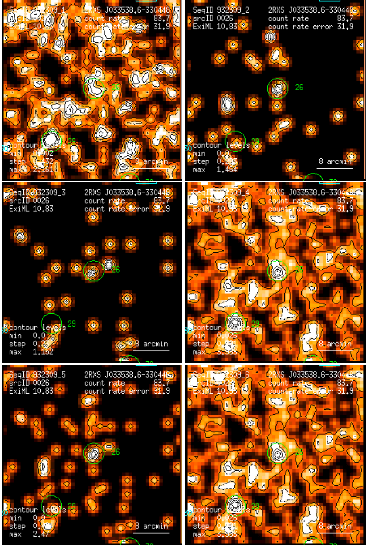
Figure 26: RASS 932309: detection 0026: band rate images, Gaussian filter: (1) PSPC channels 11 – 41, (2) 52 – 90, (3) 91 – 201, (4) 11 – 235, (5) 52 – 201, (6) 11 – 201. Broad band rates in counts/ks. Band rate contour levels in counts/ks/arcmin 2 .
