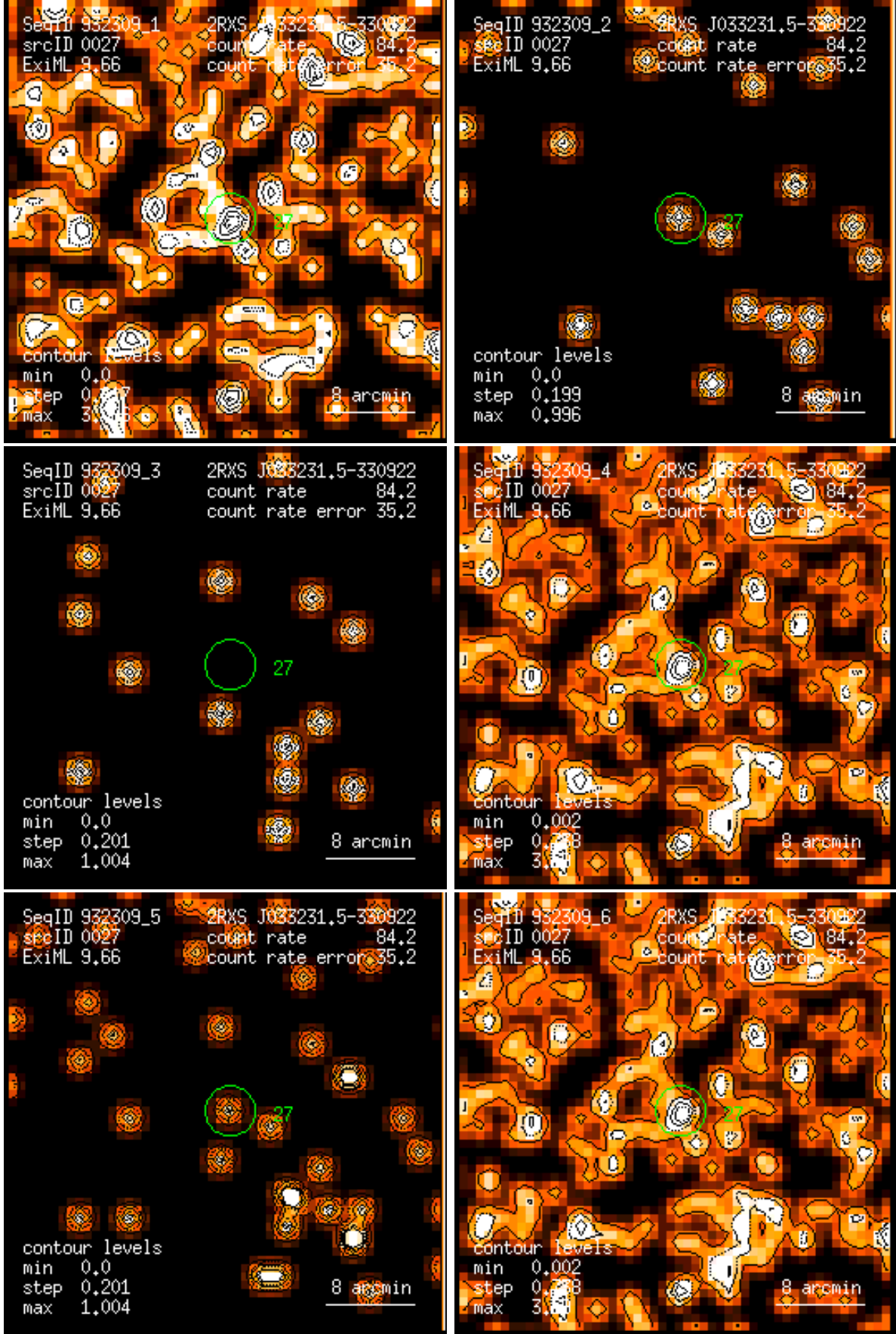
Figure 27: RASS 932309: detection 0027: band rate images, Gaussian filter: (1) PSPC channels 11 – 41, (2) 52 – 90, (3) 91 – 201, (4) 11 – 235, (5) 52 – 201, (6) 11 – 201. Broad band rates in counts/ks. Band rate contour levels in counts/ks/arcmin 2 .
