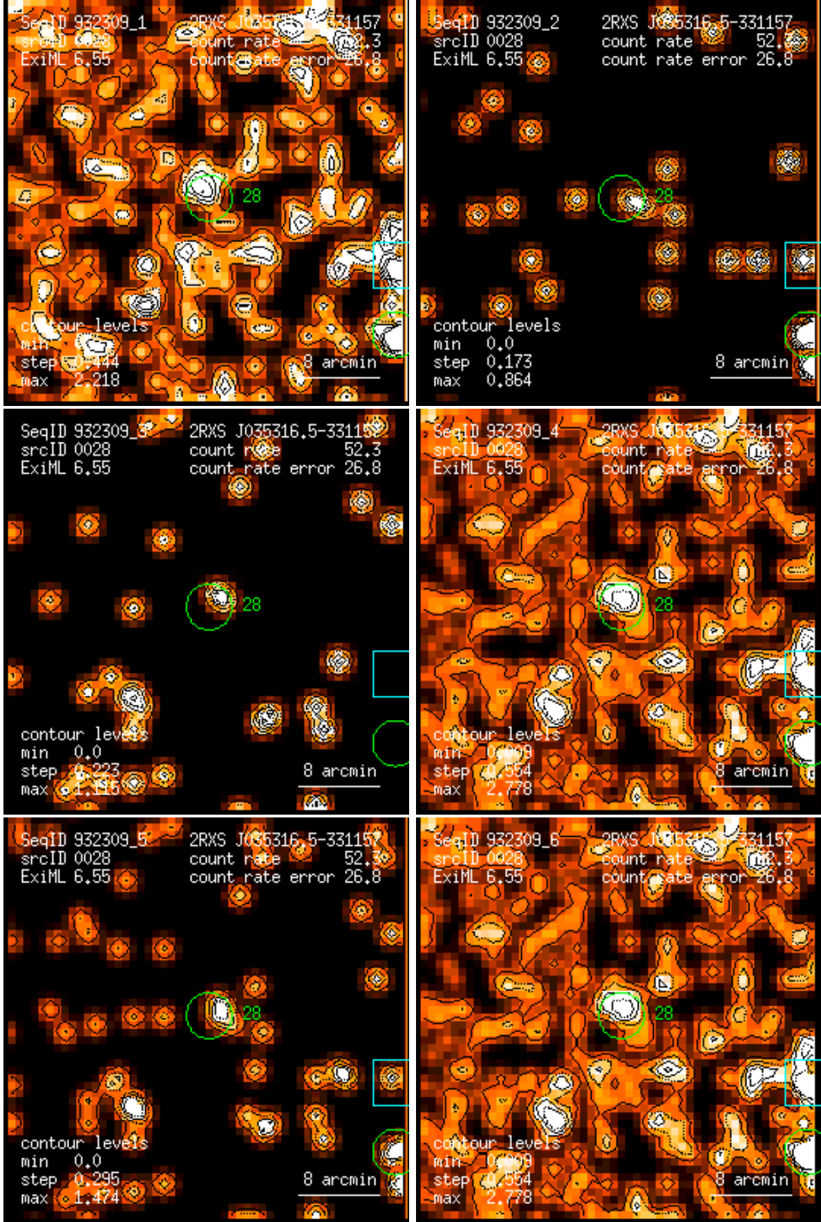
Figure 28: RASS 932309: detection 0028: band rate images, Gaussian filter: (1) PSPC channels 11 – 41, (2) 52 – 90, (3) 91 – 201, (4) 11 – 235, (5) 52 – 201, (6) 11 – 201. Broad band rates in counts/ks. Band rate contour levels in counts/ks/arcmin 2 .
