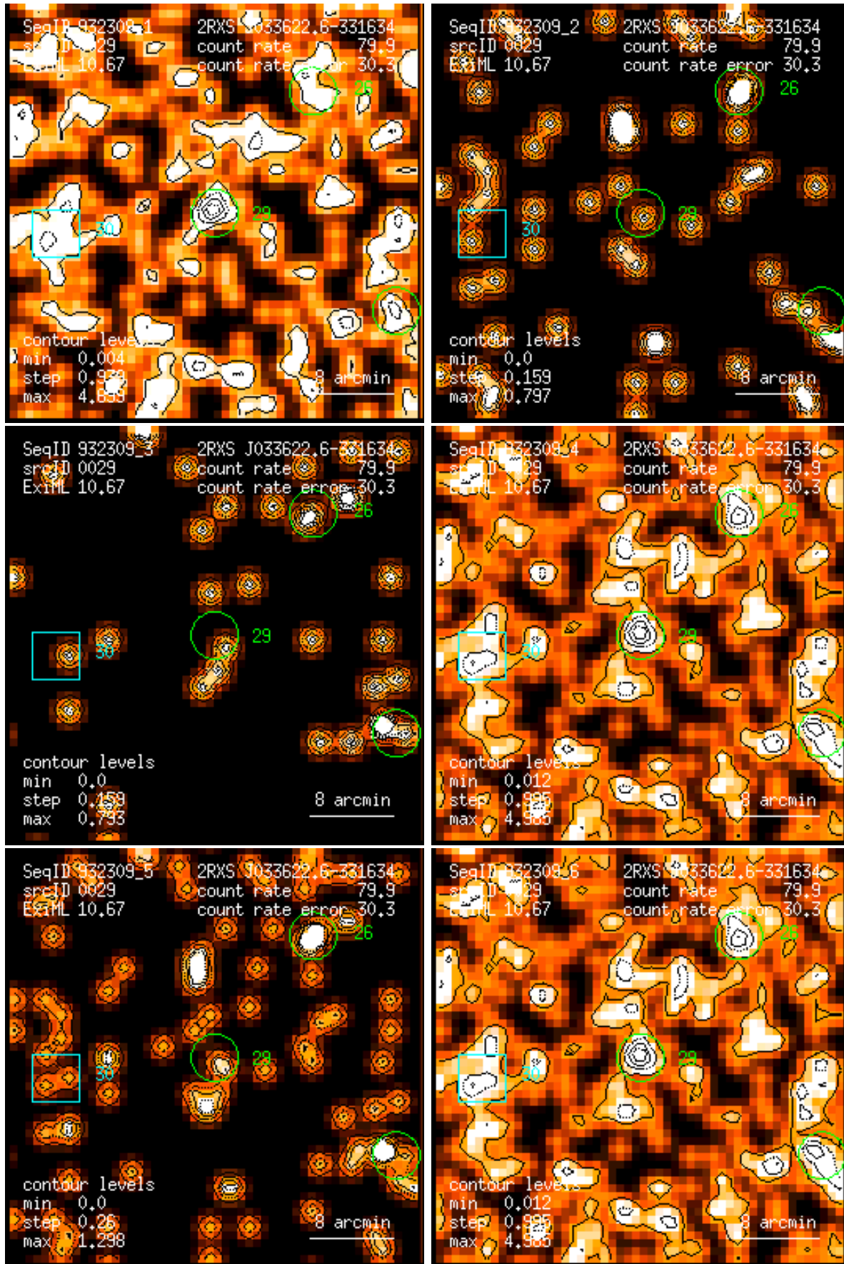
Figure 29: RASS 932309: detection 0029: band rate images, Gaussian filter: (1) PSPC channels 11 – 41, (2) 52 – 90, (3) 91 – 201, (4) 11 – 235, (5) 52 – 201, (6) 11 – 201. Broad band rates in counts/ks. Band rate contour levels in counts/ks/arcmin 2 .
