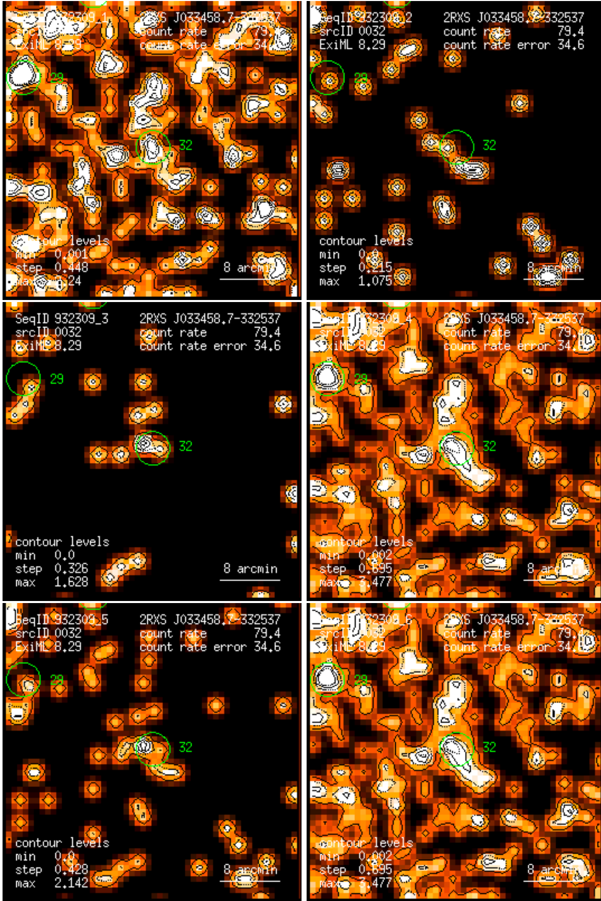
Figure 32: RASS 932309: detection 0032: band rate images, Gaussian filter: (1) PSPC channels 11 – 41, (2) 52 – 90, (3) 91 – 201, (4) 11 – 235, (5) 52 – 201, (6) 11 – 201. Broad band rates in counts/ks. Band rate contour levels in counts/ks/arcmin 2 .
