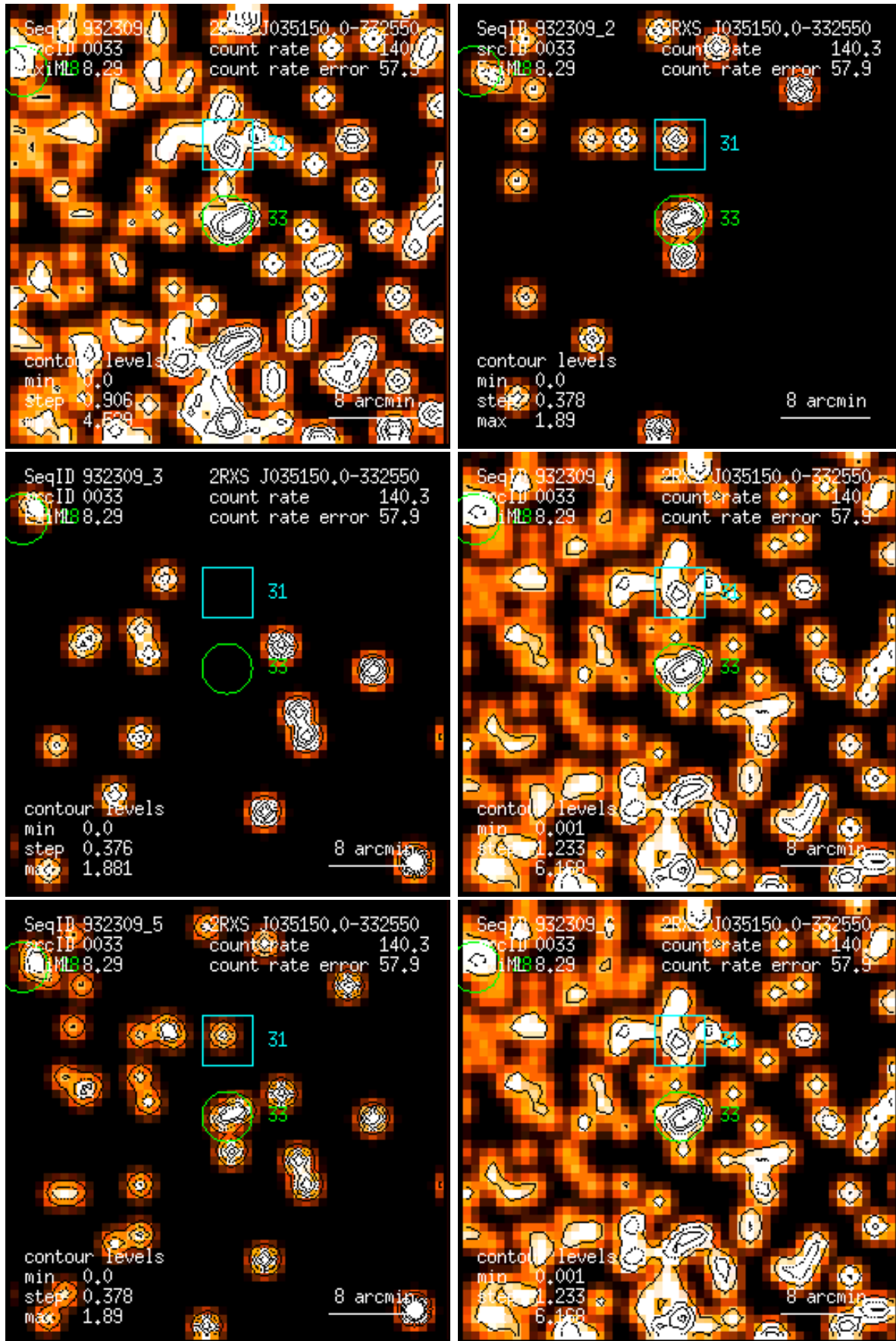
Figure 33: RASS 932309: detection 0033: band rate images, Gaussian filter: (1) PSPC channels 11 – 41, (2) 52 – 90, (3) 91 – 201, (4) 11 – 235, (5) 52 – 201, (6) 11 – 201. Broad band rates in counts/ks. Band rate contour levels in counts/ks/arcmin 2 .
