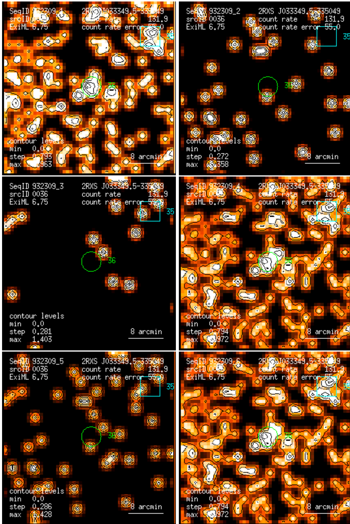
Figure 36: RASS 932309: detection 0036: band rate images, Gaussian filter: (1) PSPC channels 11 – 41, (2) 52 – 90, (3) 91 – 201, (4) 11 – 235, (5) 52 – 201, (6) 11 – 201. Broad band rates in counts/ks. Band rate contour levels in counts/ks/arcmin 2 .
