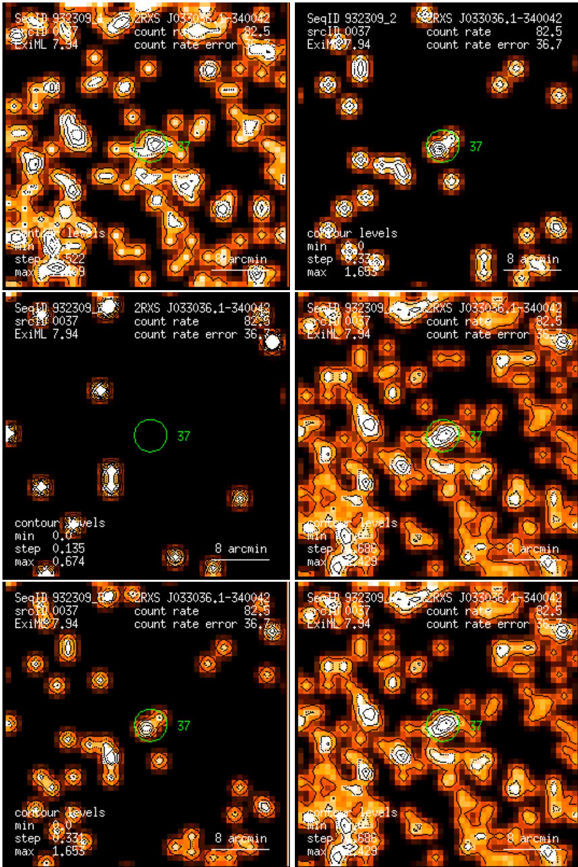
Figure 37: RASS 932309: detection 0037: band rate images, Gaussian filter: (1) PSPC channels 11 – 41, (2) 52 – 90, (3) 91 – 201, (4) 11 – 235, (5) 52 – 201, (6) 11 – 201. Broad band rates in counts/ks. Band rate contour levels in counts/ks/arcmin 2 .
