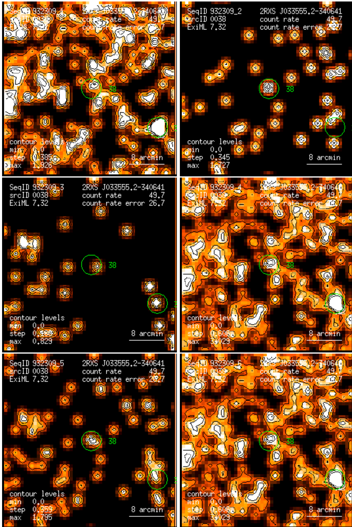
Figure 38: RASS 932309: detection 0038: band rate images, Gaussian filter: (1) PSPC channels 11 – 41, (2) 52 – 90, (3) 91 – 201, (4) 11 – 235, (5) 52 – 201, (6) 11 – 201. Broad band rates in counts/ks. Band rate contour levels in counts/ks/arcmin 2 .
